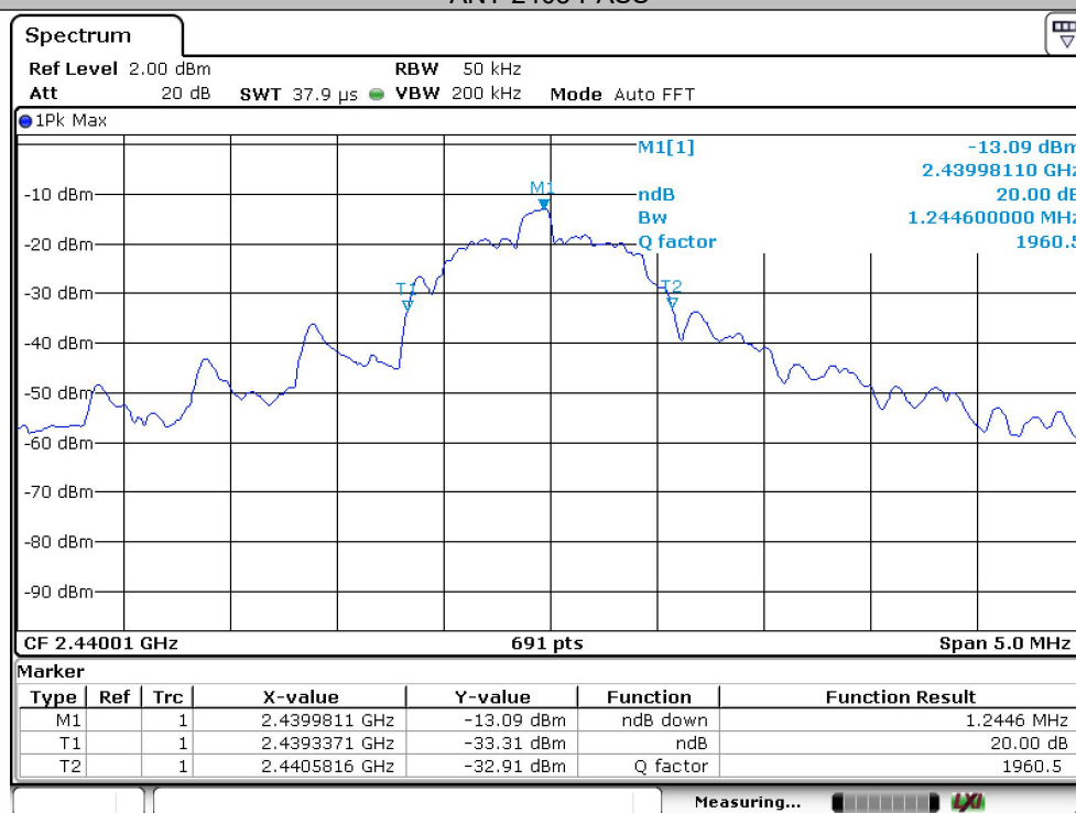
ANT-2440-PASS
