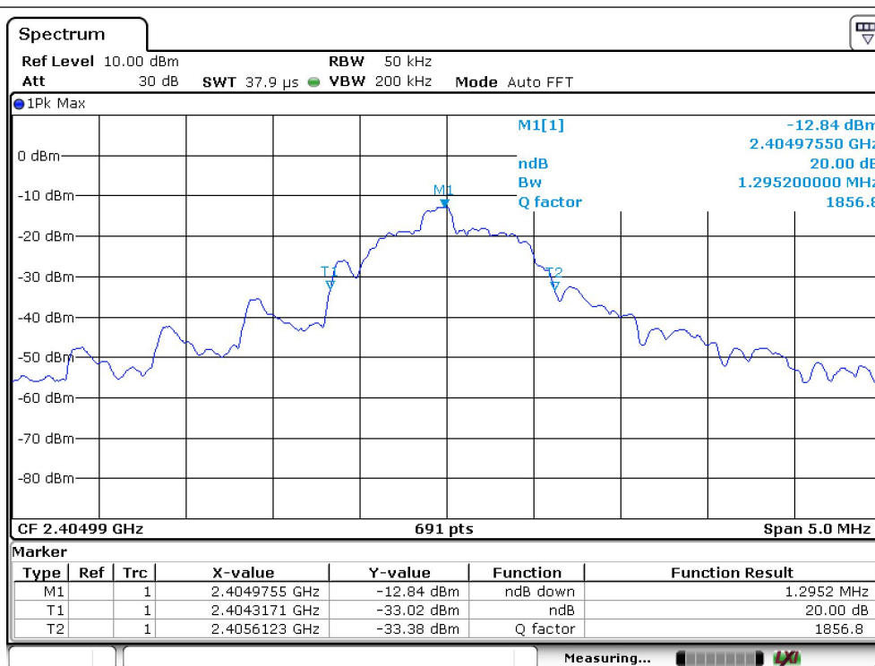
ANT-2405-PASS
