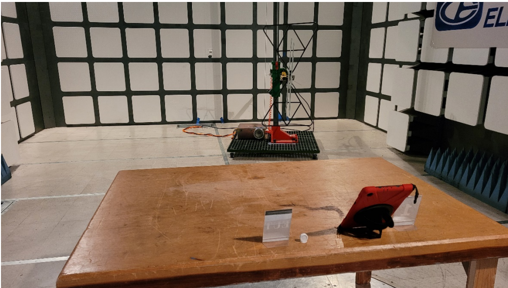
Radiated Emissions HF Rear
