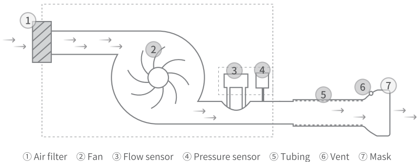
Figure 3-3 Device airflow schematic
