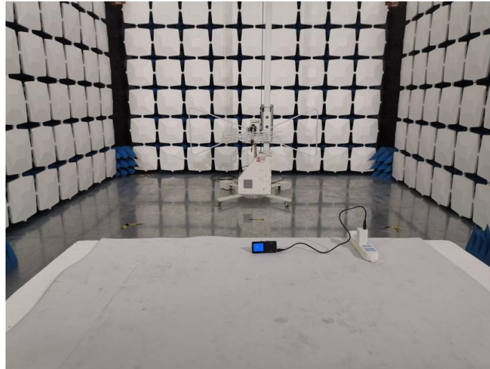
Above 1GHz for radiated emission test setup
