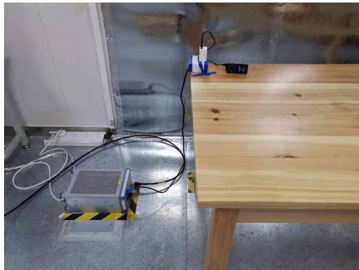
Conducted emission test setup
