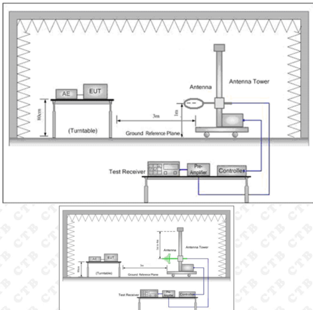
Figure 1. Below 30MHz
