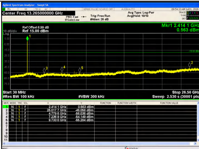
RF Conducted Spurious Emissions Graphs
