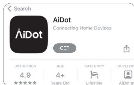
Download Interface
