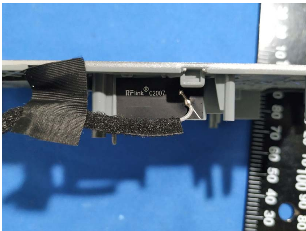
WiFi ANT Chain 0
