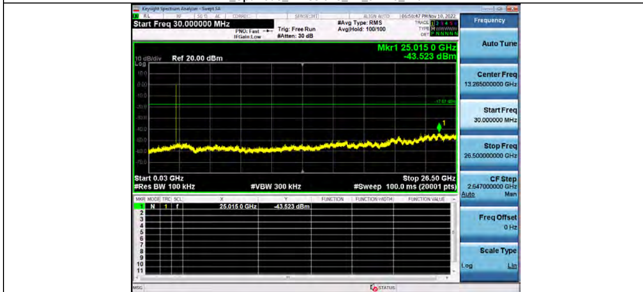
2 Spurious Emissions BT 3-DH5 2402
