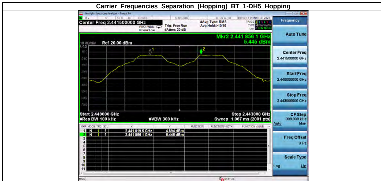
Carrier_Frequencies_Separation_(Hopping)_BT_1-DH5_Hopping
