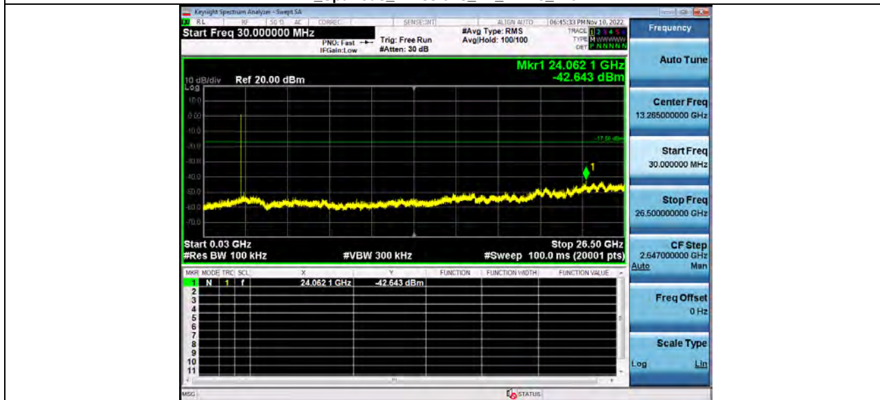
2 Spurious Emissions BT 2-DH5 2402
