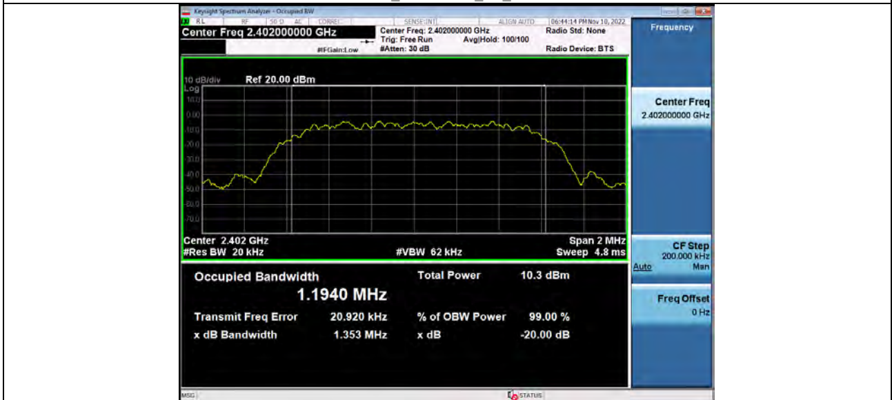
-20dB_Bandwidth_BT_2402
