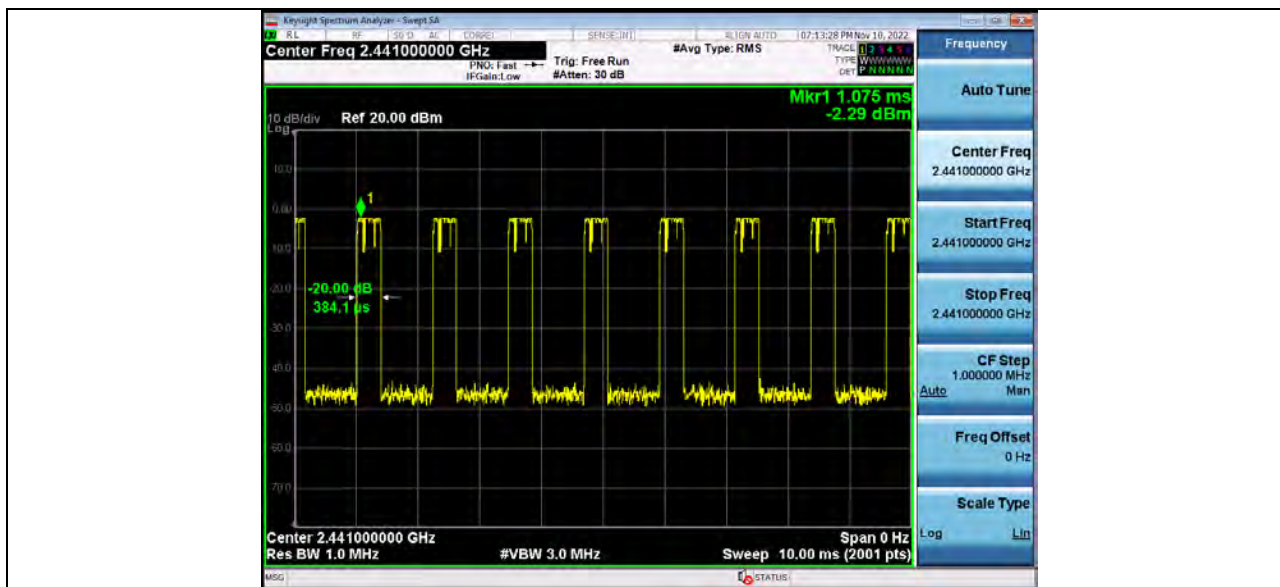
Dwell_Time (Hopping) BT 2-DH5 2441 One Burst Time
