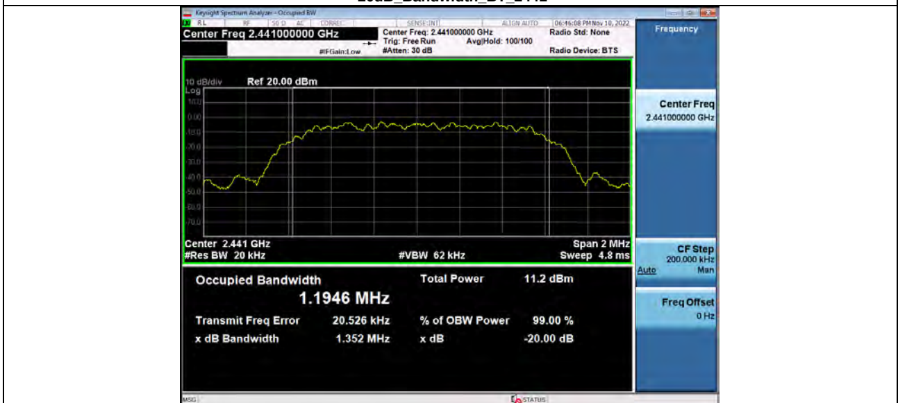
-20dB_Bandwidth_BT_2441
