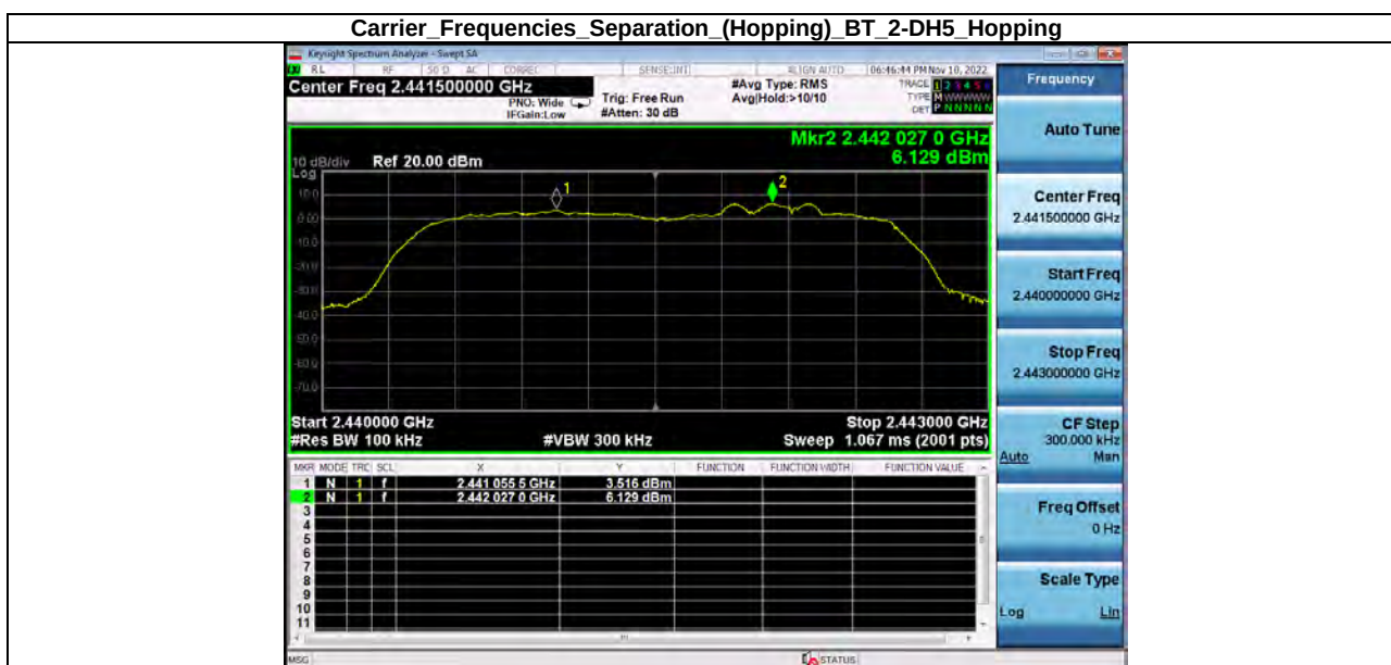
Carrier_Frequencies_Separation_(Hopping)_BT_2-DH5_Hopping
