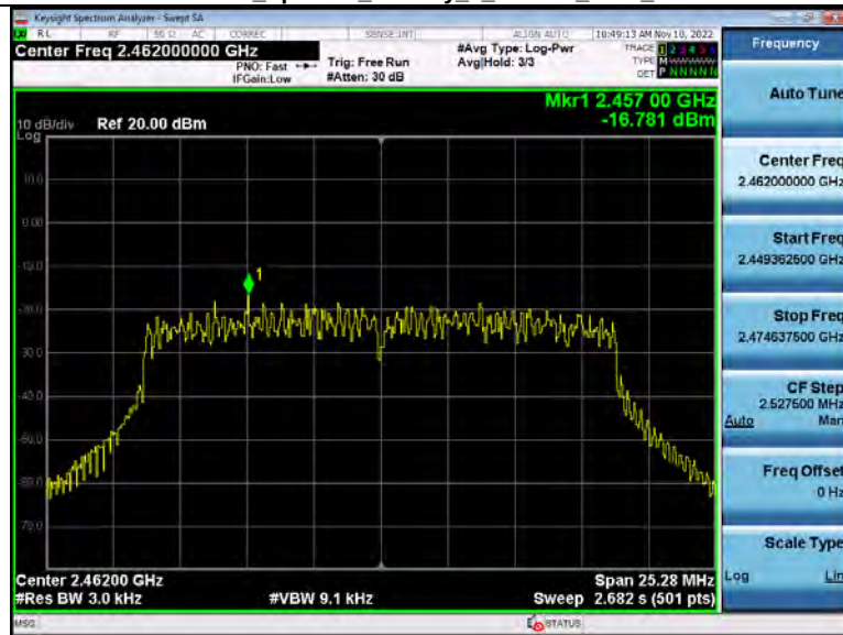
Power Spectral Density_2_4GWiFi_2462_00
