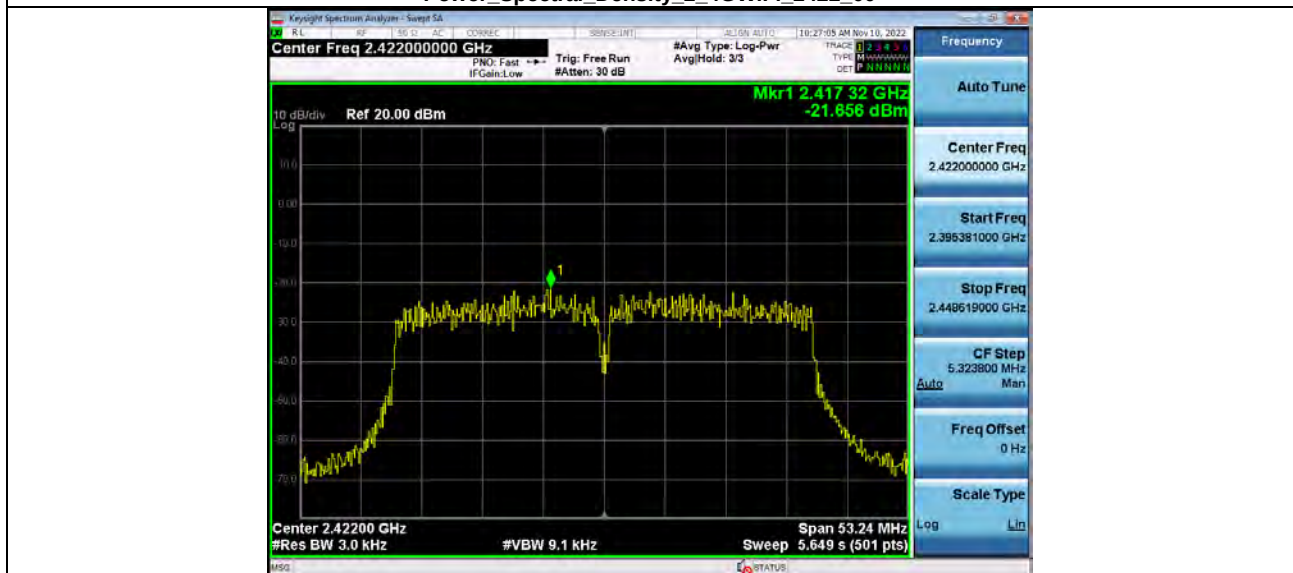
Power_Spectral_Density_2_4GWiFi_2422_00
