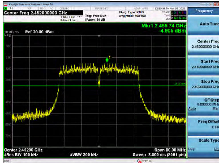
2 Spurious Emission 2 4GWiFi NVNT ANT1 802 11n(HT40) 2452 00
