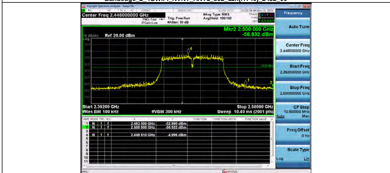
Bandedge 2 4GWiFi_NVNT_ANT1_802_11n(HT40)_2452_00
