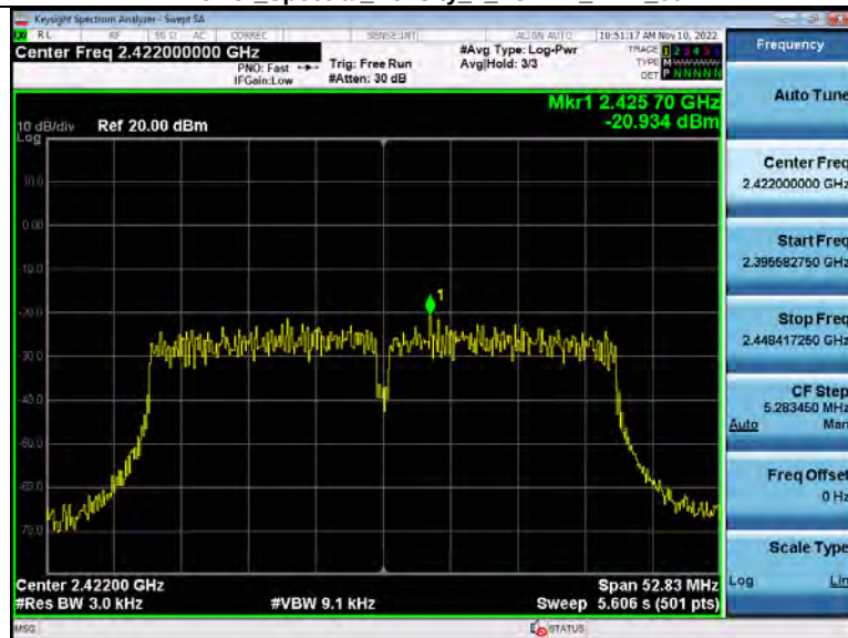
Power Spectral Density_2_4GWiFi_2422_00
