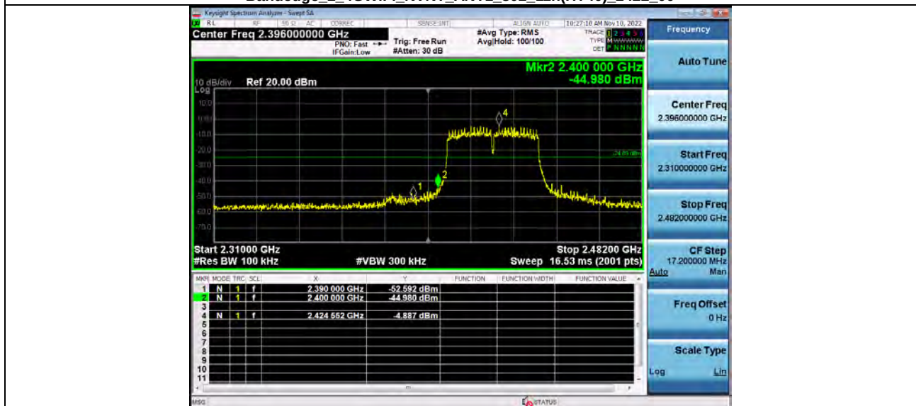
Bandedge 2 4GWiFi_NVNT_ANT1_802_11n(HT40)_2422_00
