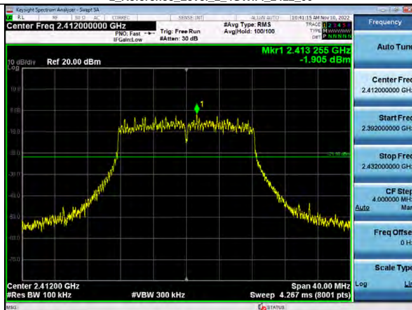
2 Spurious Emission 2 4GWiFi_NVNT ANT1 802_11g 2412_00
