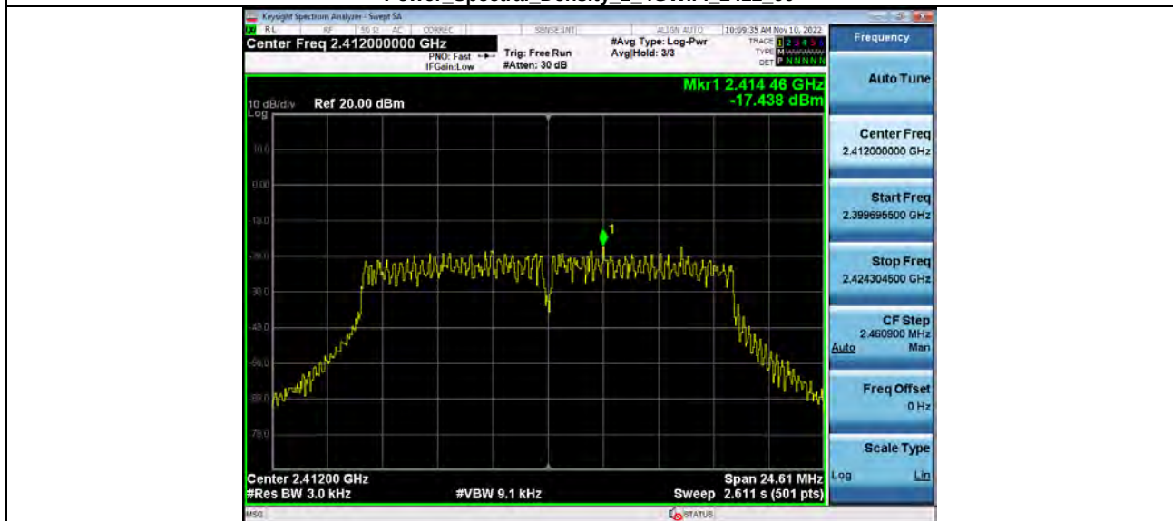
Power_Spectral_Density_2_4GWiFi_2412_00
