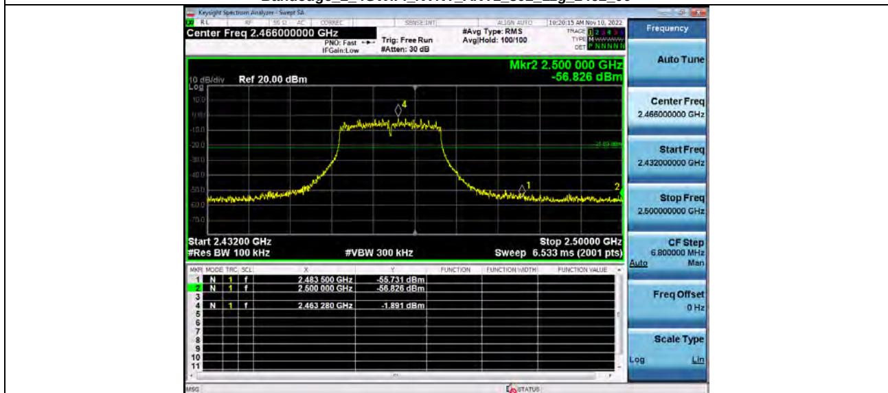
Bandedge_2_4GWiFi_NVNT_ANT1_802_11g_2462_00
