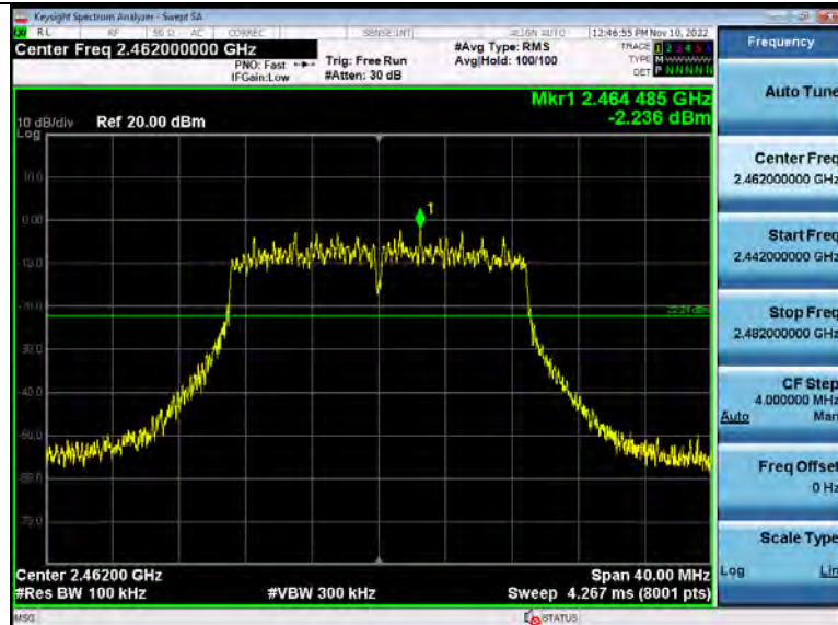
2 Spurious Emission 2 4GWiFi NVNT ANT1 802 11n(HT20) 2462 00
