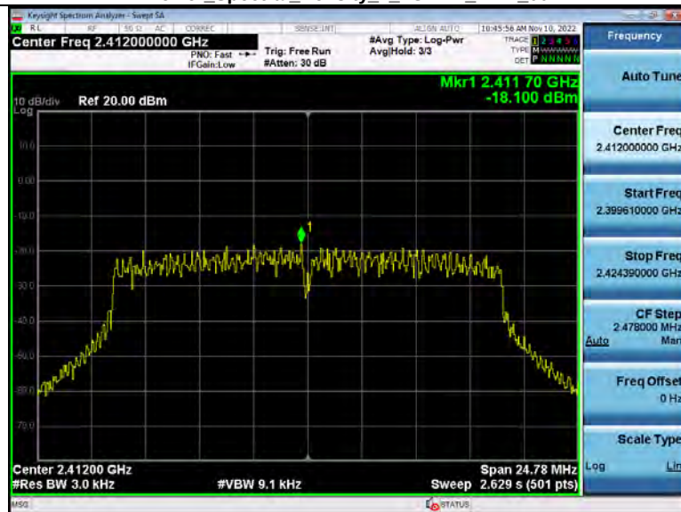
Power Spectral Density_2_4GWiFi_2412_00
