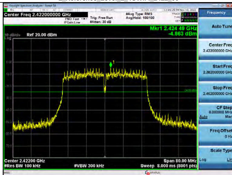
2 Spurious Emission 2 4GWiFi NVNT ANT1 802 11n(HT40) 2422 00
