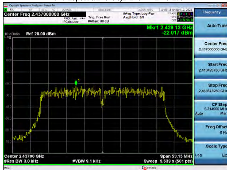
Power Spectral Density_2_4GWiFi_2437_00
