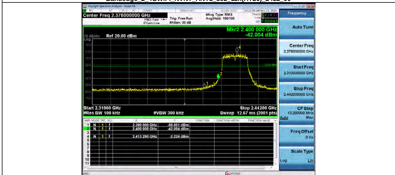
Bandedge_2_4GWiFi_NVNT_ANT1_802_11n(HT20)_2412_00
