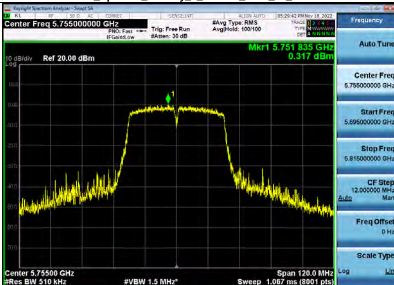
Power Spectral Density 5_8WiFi 5755_00 40M.PNG
