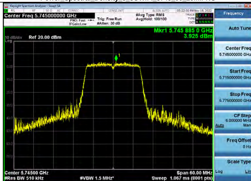
Power Spectral Density 5_8GWiFi_5745_00_20M.PNG
