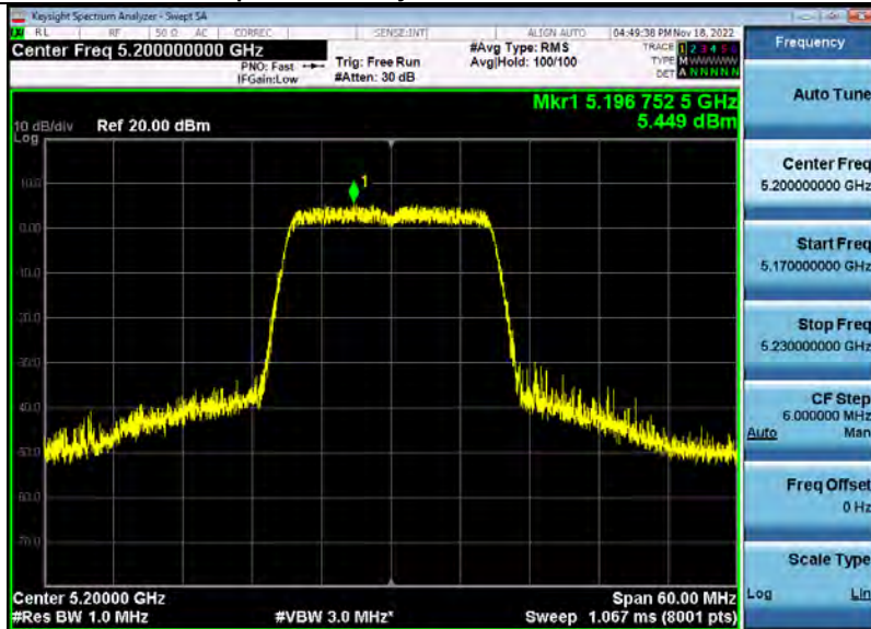
Power Spectral Density 5 2GWiFi 5200 00 20M.PNG
