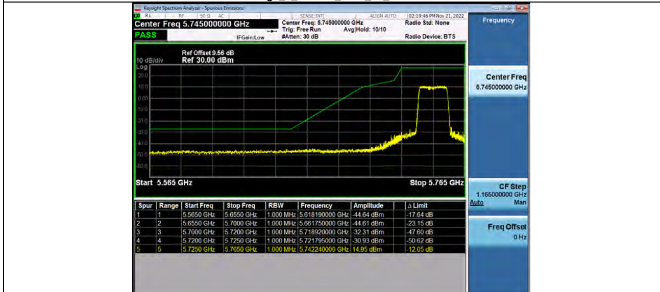
Bandedge_5_8WiFi_5745_00_20M.PNG
