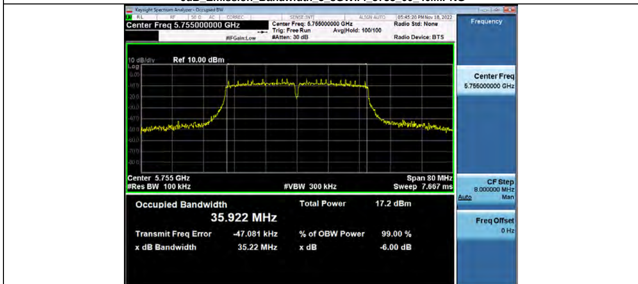
-6dB Emission Bandwidth 5_8WiFi 5755_00_40M.PNG
