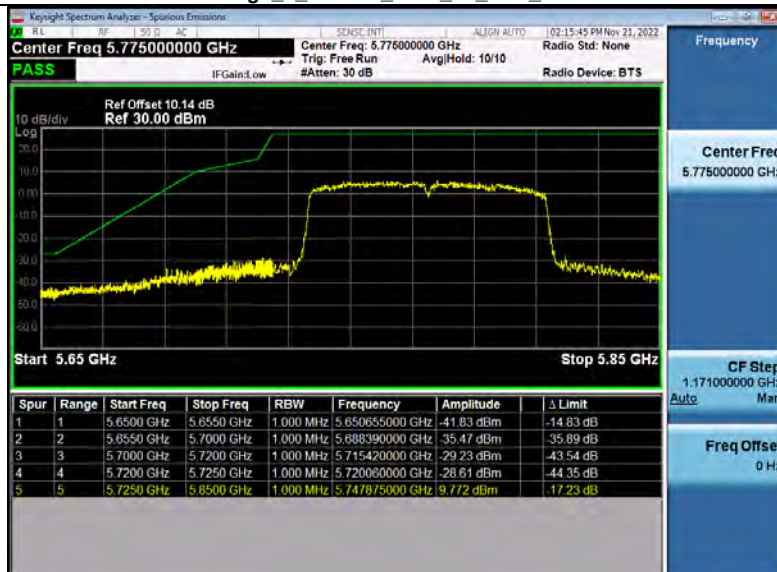
Bandedge_5_8WiFi_5775_00_80M_low.PNG
