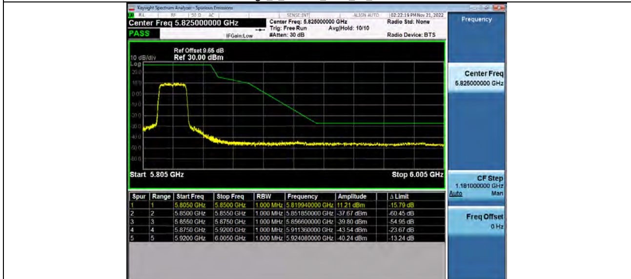
Bandedge_5_8WiFi_5825_00_20M.PNG
