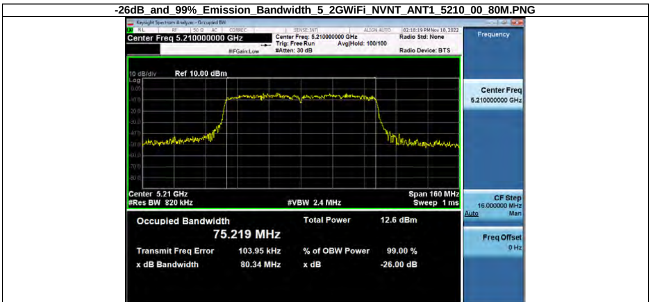
-26dB and 99% Emission Bandwidth 5 2GWiFi NVNT ANT1 5210_00 80M.PNG
