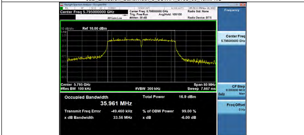
-6dB Emission Bandwidth 5_8WiFi 5795_00_40M.PNG
