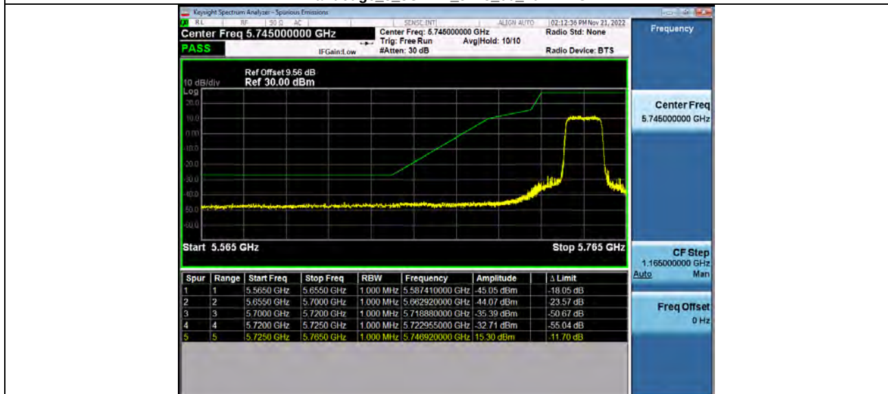
Bandedge_5_8WiFi_5745_00_20M.PNG
