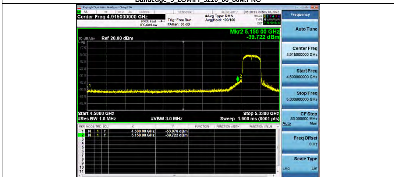
Bandedge_5_2GWiFi_5210_00_80M.PNG
