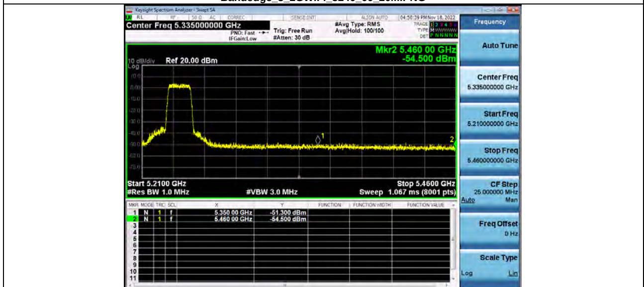
Bandedge_5_2GWiFi_5240_00_20M.PNG
