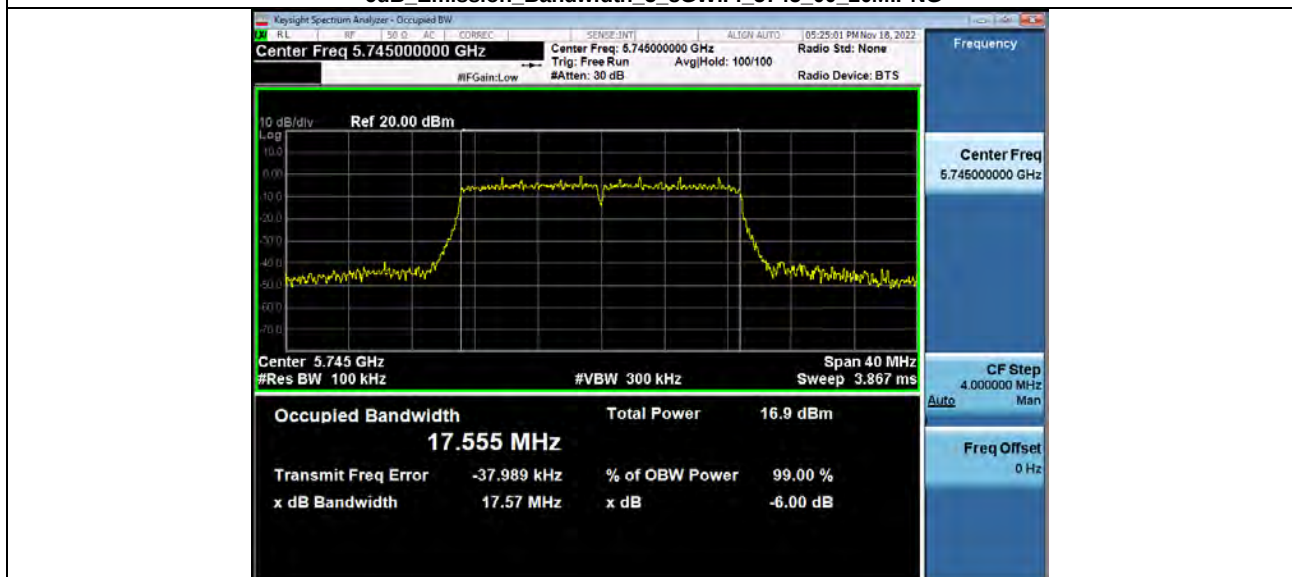
-6dB Emission Bandwidth 5_8WiFi 5745_00_20M.PNG
