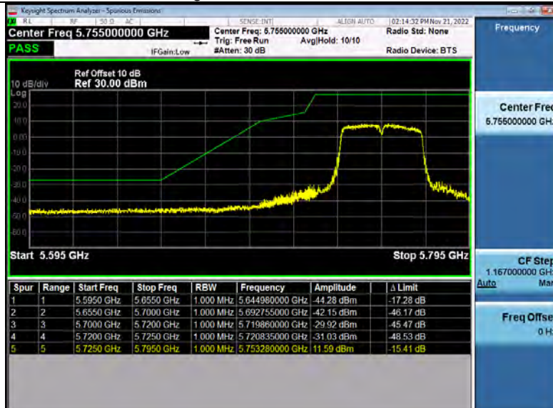
Bandedge_5_8GWiFi_5755_00_40M.PNG
