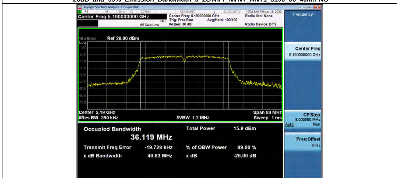
-26dB and 99% Emission Bandwidth 5 2GWiFi NVNT ANT1 5190_00_40M.PNG
