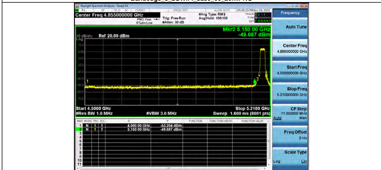
Bandedge_5_2GWiFi_5180_00_20M.PNG
