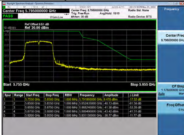
Bandedge_5_8WiFi_5795_00_40M.PNG
