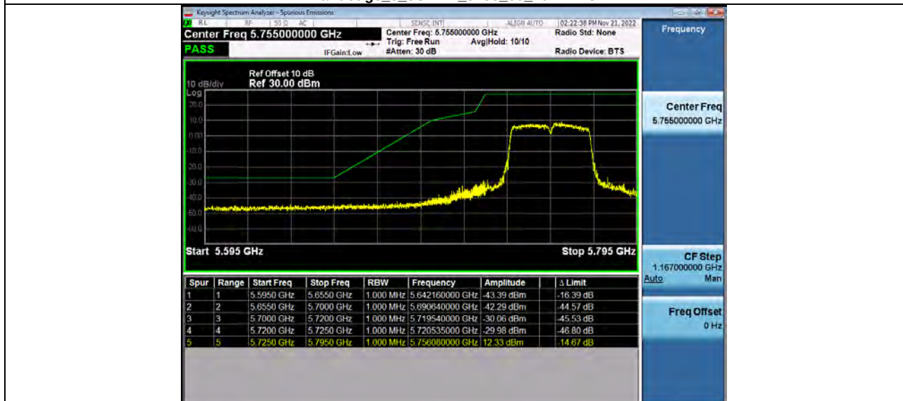
Bandedge_5_8WiFi_5755_00_40M.PNG
