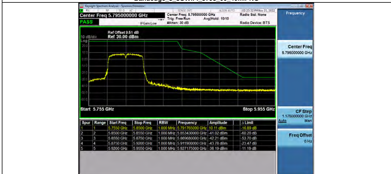
Bandedge_5_8WiFi_5795_00_40M.PNG
