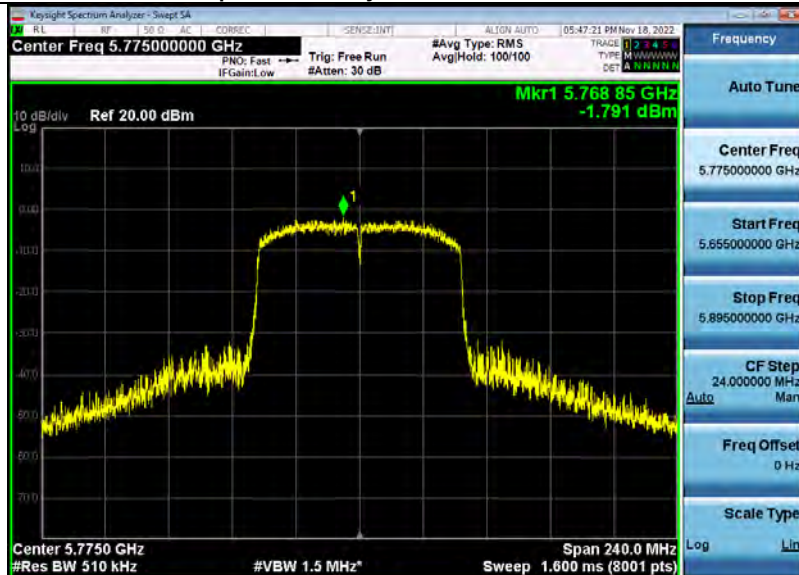
Power Spectral Density 5 8WiFi 5775 00 80M.PNG
