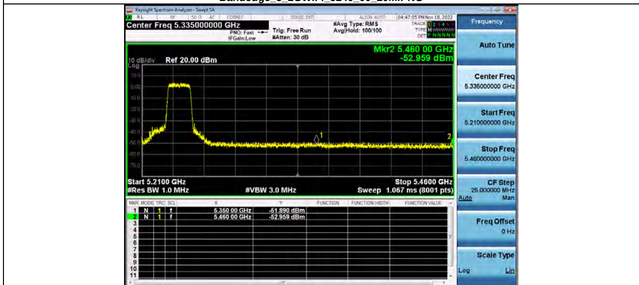
Bandedge_5_2GWiFi_5240_00_20M.PNG
