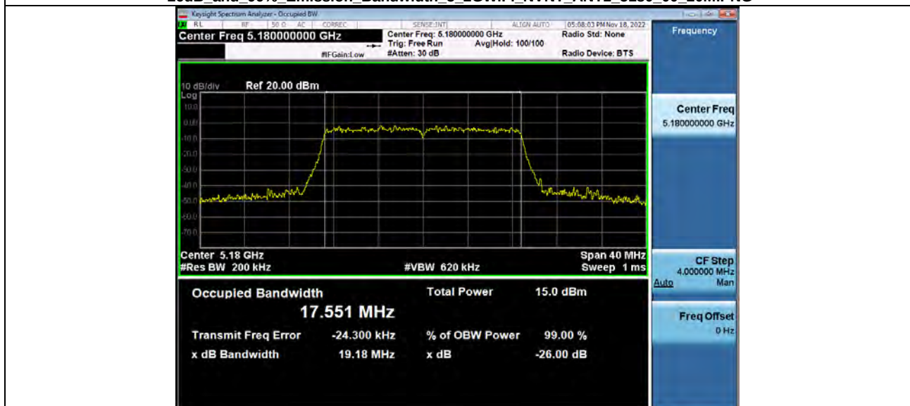
-26dB and 99% Emission Bandwidth 5 2GWiFi NVNT ANT1 5180_00 20M.PNG
