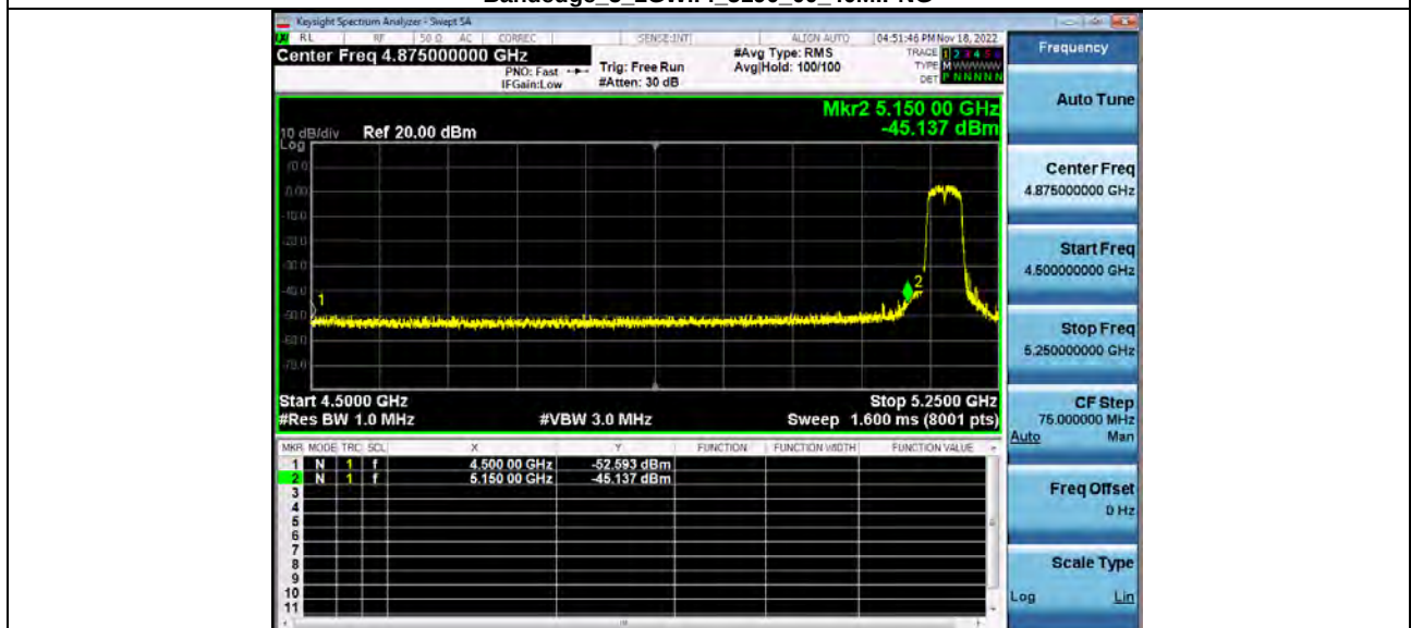
Bandedge_5_2GWiFi_5190_00_40M.PNG
