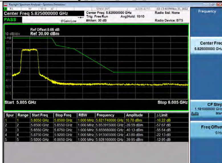
Bandedge_5_8WiFi_5825_00_20M.PNG
