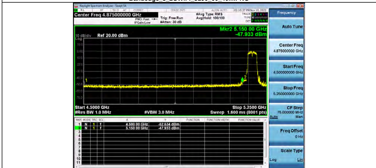
Bandedge_5_2GWiFi_5190_00_40M.PNG
