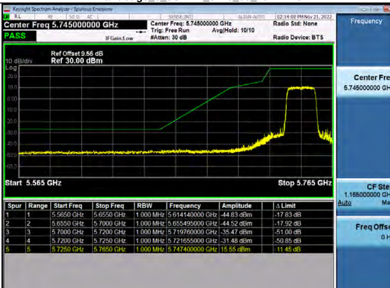
Bandedge_5_8WiFi_5745_00_20M.PNG
