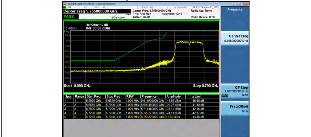
Bandedge_5_8WiFi_5755_00_40M.PNG
