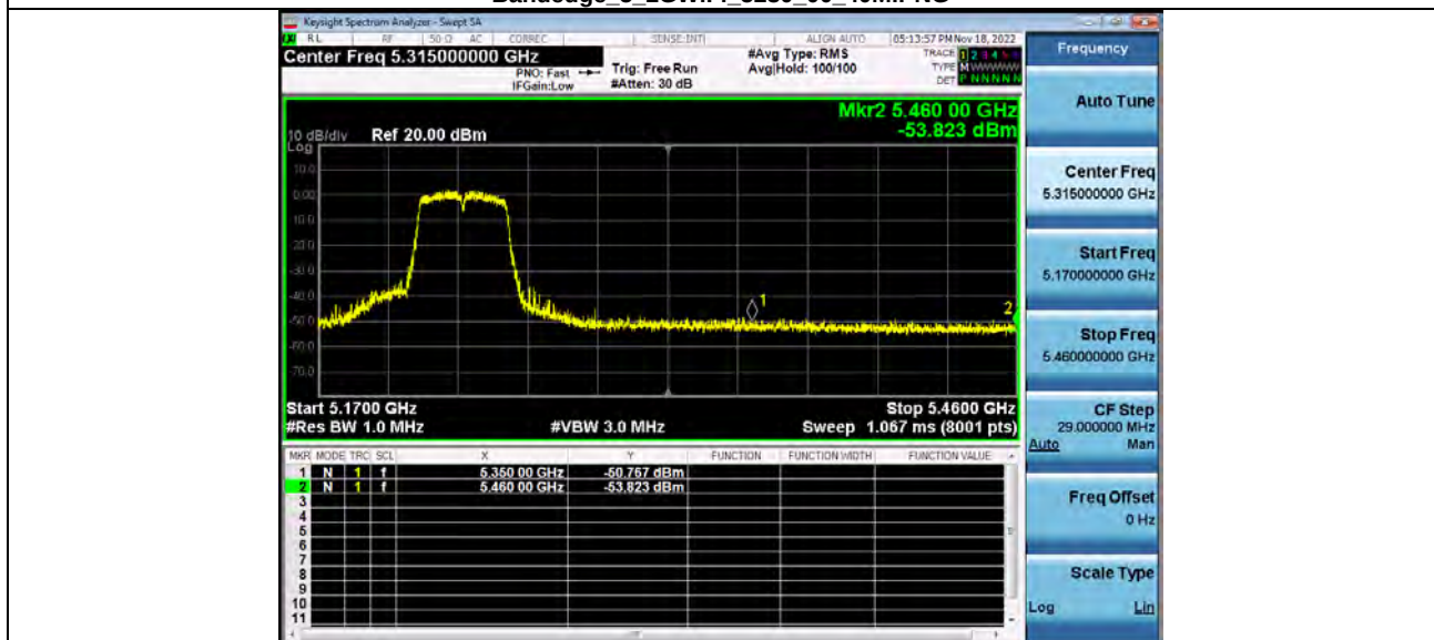
Bandedge_5_2GWiFi_5230_00_40M.PNG
