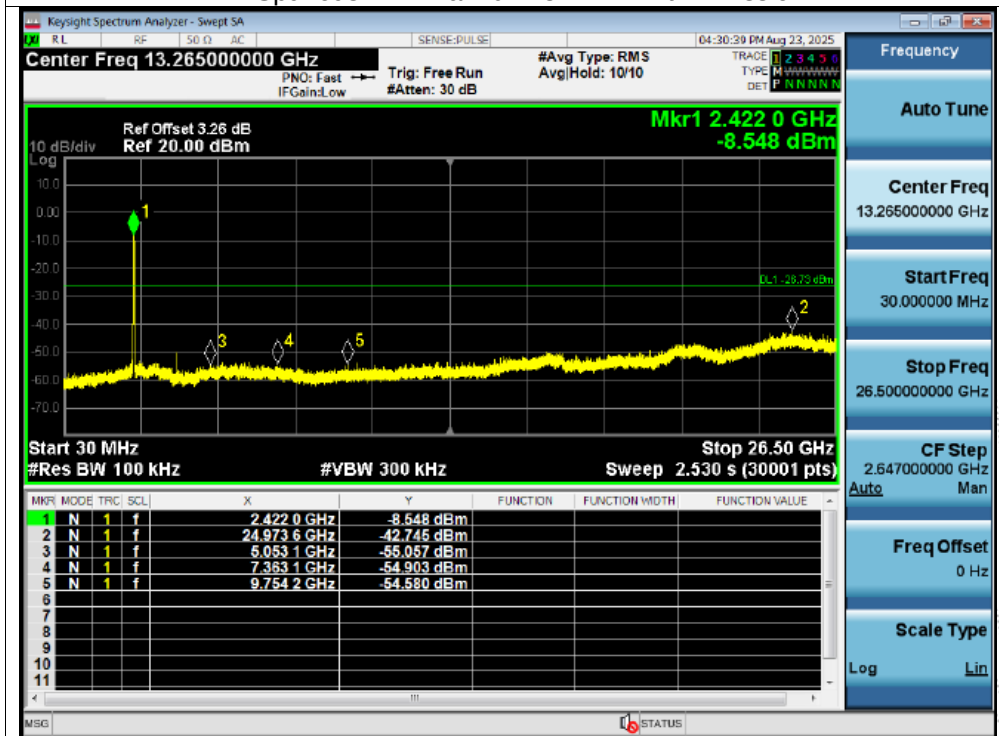
Tx. Spurious NVNT ax40 2437MHz Ant1 Emission
