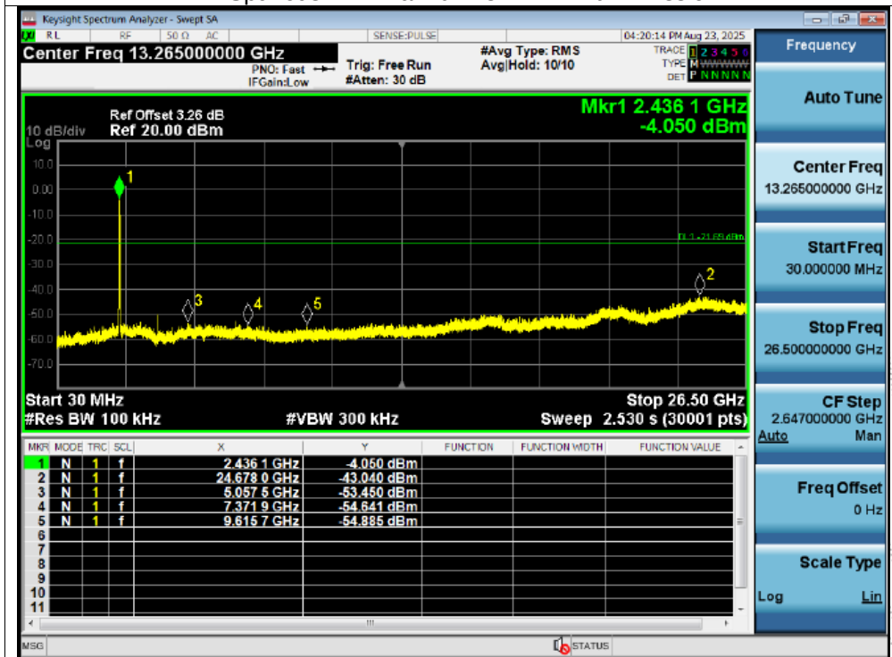
Tx. Spurious NVNT ax20 2437MHz Ant1 Emission
