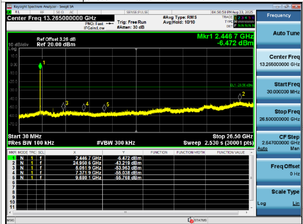
Tx. Spurious NVNT ax40 2452MHz Ant1 Emission
