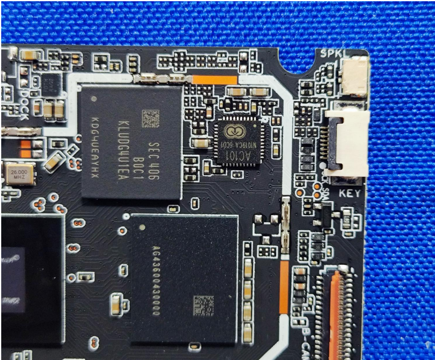
Internal photograph of EUT
