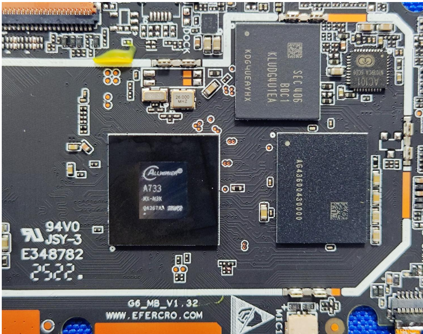
Internal photograph of EUT
