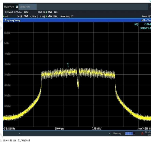
11N40SISO-Ant1-2422-PASS
