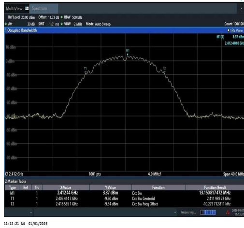
11B-Ant1-2412
