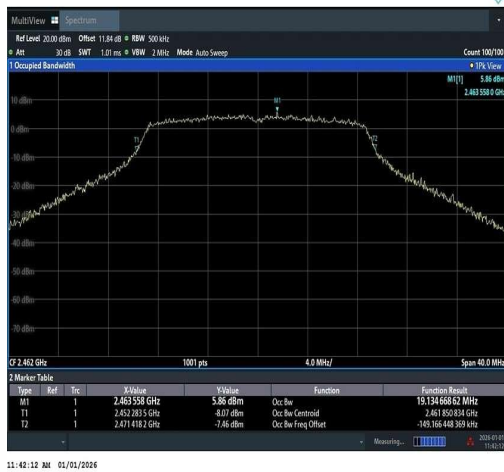
11N20SISO-Ant1-2462
