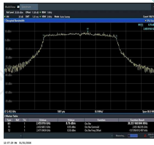
11AX40SISO-Ant1-2452
