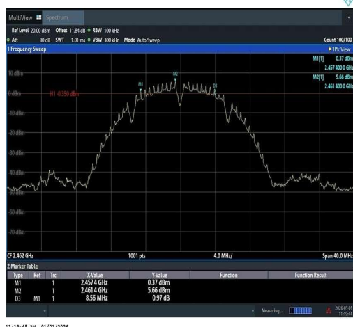
11B-Ant1-2462-PASS
