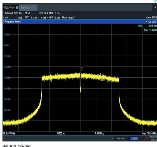
11AX40SISO-Ant1-2437-PASS
