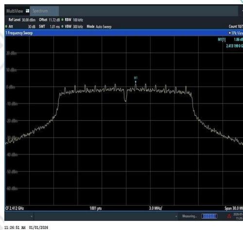
11G-Ant1-2412-0~Reference-PASS
