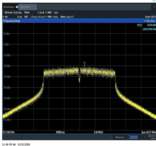
11N20SISO-Ant1-2462-PASS
