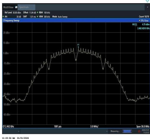
11B-Ant1-2462-0~Reference-PASS
