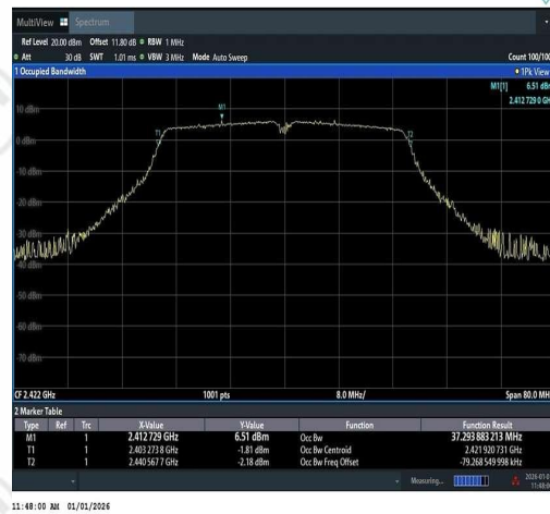
11N40SISO-Ant1-2422
