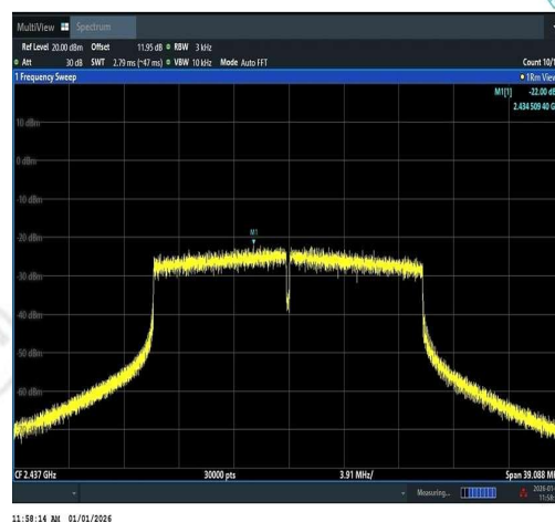
11AX20SISO-Ant1-2437-PASS
