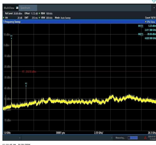
11B-Ant1-2412-1000~26500-PASS
