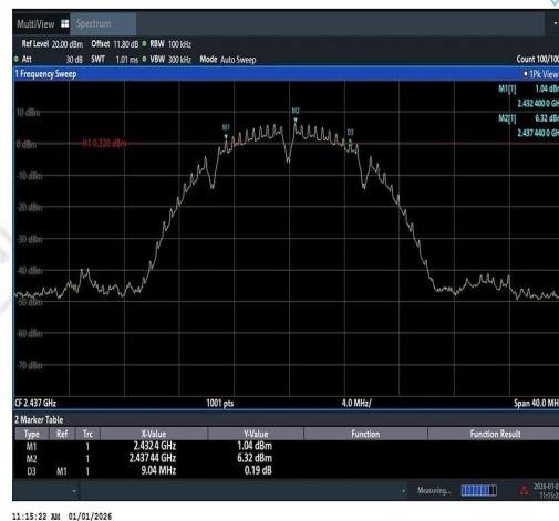
11B-Ant1-2437-PASS
