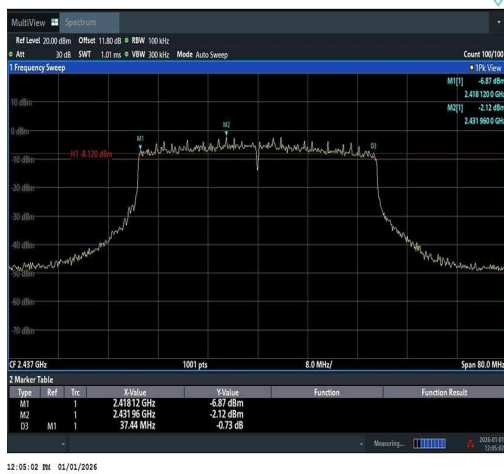
11AX40SISO-Ant1-2437-PASS
