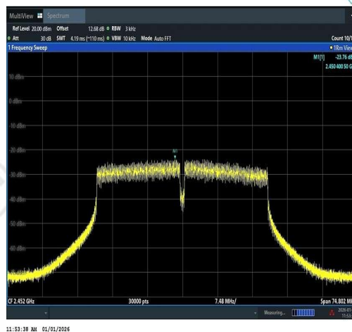
11N40SISO-Ant1-2452-PASS
