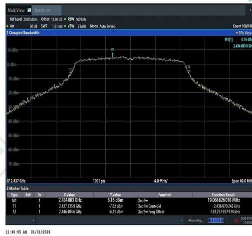
11N20SISO-Ant1-2437
