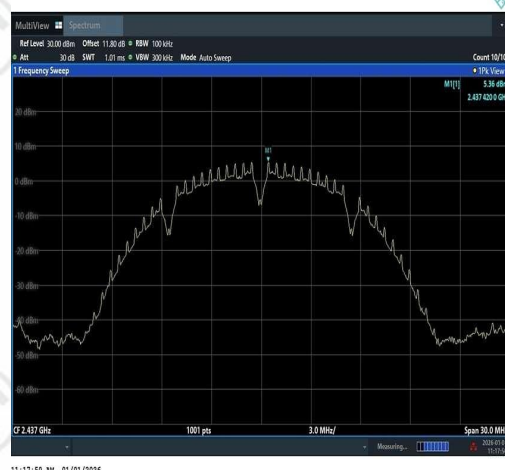
11B-Ant1-2437-0~Reference-PASS
