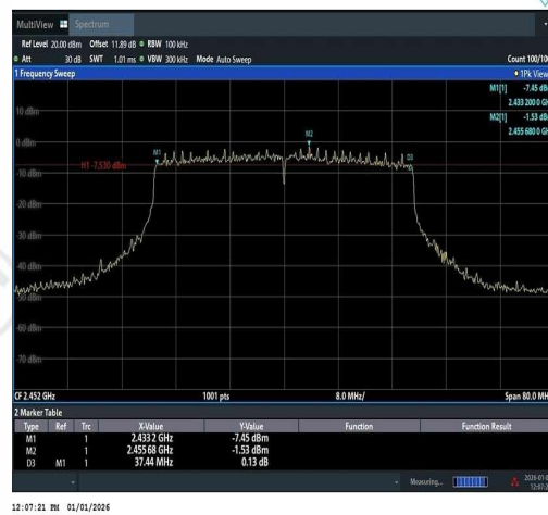
11AX40SISO-Ant1-2452-PASS
