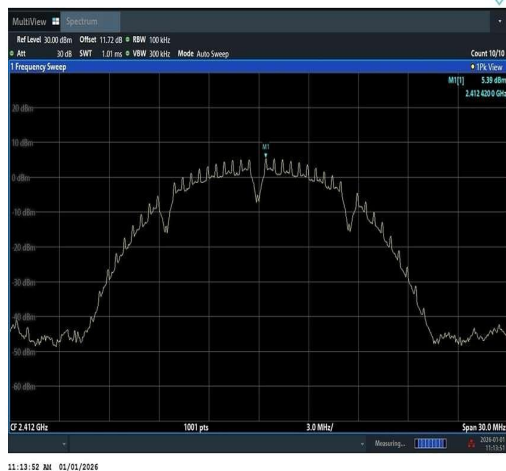
11B-Ant1-2412-0~Reference-PASS
