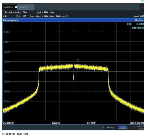
11AX20SISO-Ant1-2462-PASS
