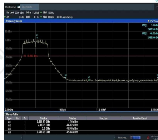
11N20SISO-Ant1-2462-PASS
