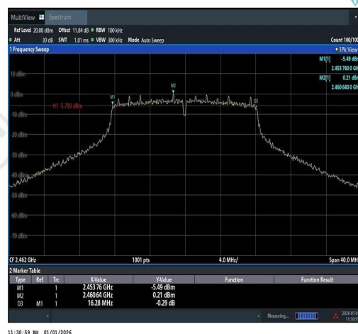
11G-Ant1-2462-PASS
