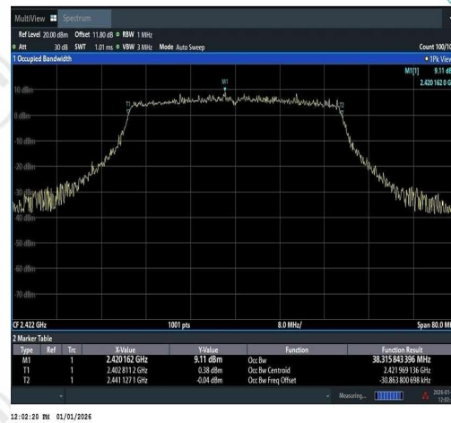
11AX40SISO-Ant1-2422
