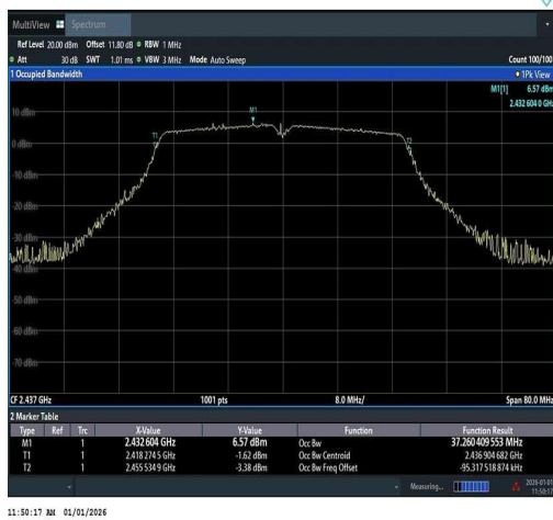
11N40SISO-Ant1-2437
