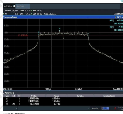
11G-Ant1-2412-PASS
