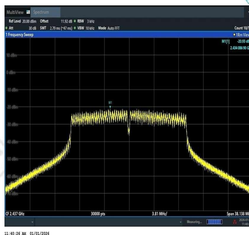
11N20SISO-Ant1-2437-PASS
