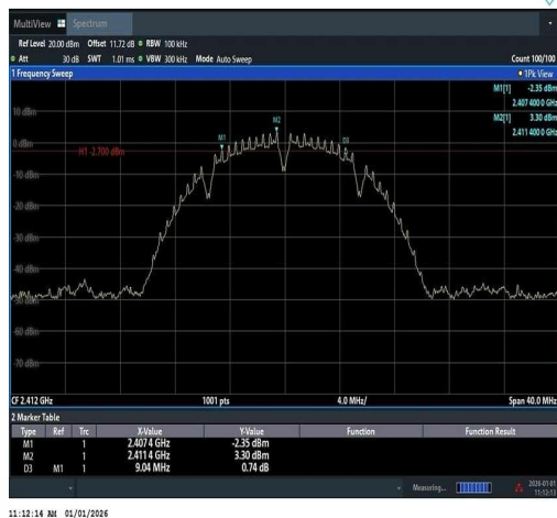
11B-Ant1-2412-PASS
