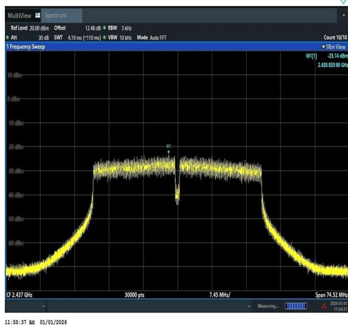
11N40SISO-Ant1-2437-PASS
