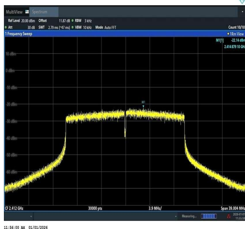
11AX20SISO-Ant1-2412-PASS
