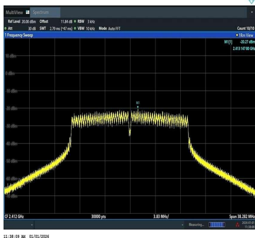
11N20SISO-Ant1-2412-PASS
