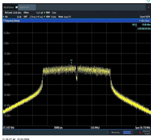
11G-Ant1-2437-PASS
