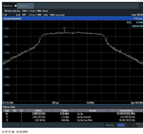
11N20SISO-Ant1-2412
