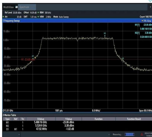
11AX40SISO-Ant1-5510
