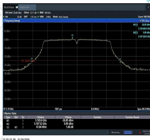
11AC40SISO-Ant1-5190
