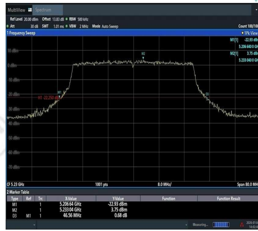
11AX40SISO-Ant1-5230
