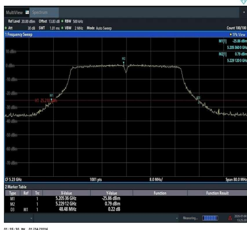
11AC40SISO-Ant1-5230
