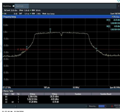
11AC40SISO-Ant1-5270
