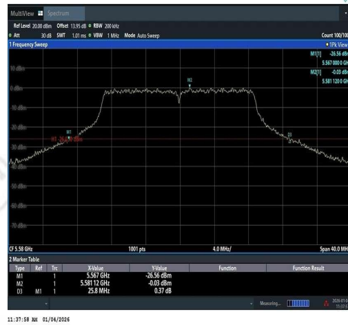
11N20SISO-Ant1-5580
