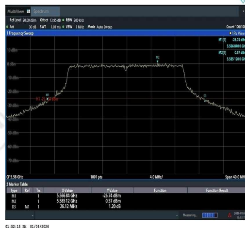
11AX20SISO-Ant1-5580
