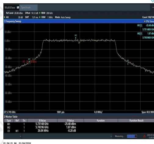
11AX20SISO-Ant1-5745
