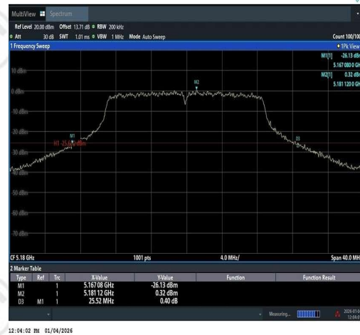
11AC20SISO-Ant1-5180
