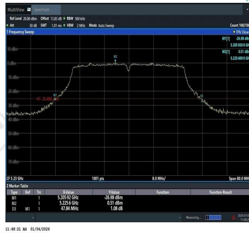
11N40SISO-Ant1-5230
