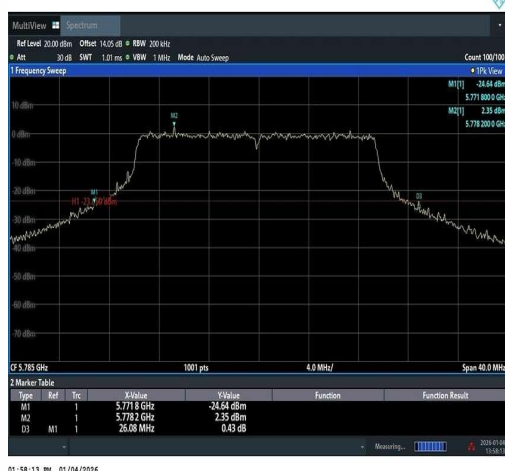
11AX20SISO-Ant1-5785
