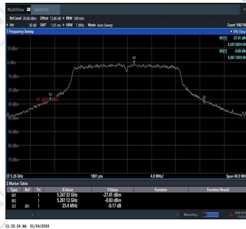
11N20SISO-Ant1-5260
