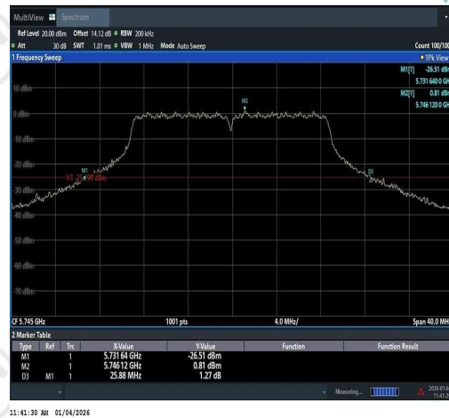
11N20SISO-Ant1-5745
