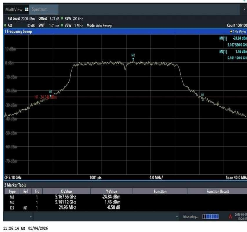
11N20SISO-Ant1-5180
