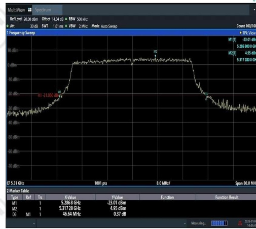
11AX40SISO-Ant1-5310
