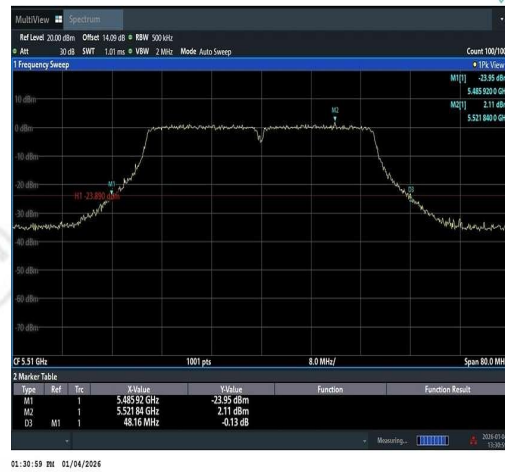
11AC40SISO-Ant1-5510
