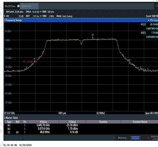
11AC40SISO-Ant1-5670
