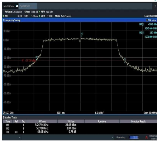
11AX40SISO-Ant1-5270
