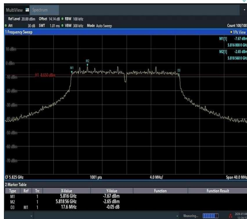
11AC20SISO-Ant1-5825-PASS
