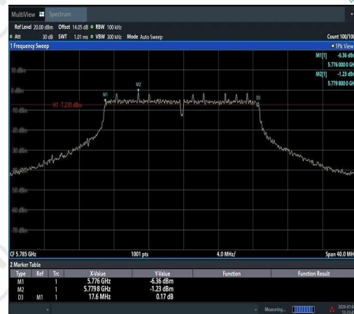
11AC20SISO-Ant1-5785-PASS
