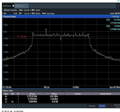
11AX20SISO-Ant1-5785-PASS
