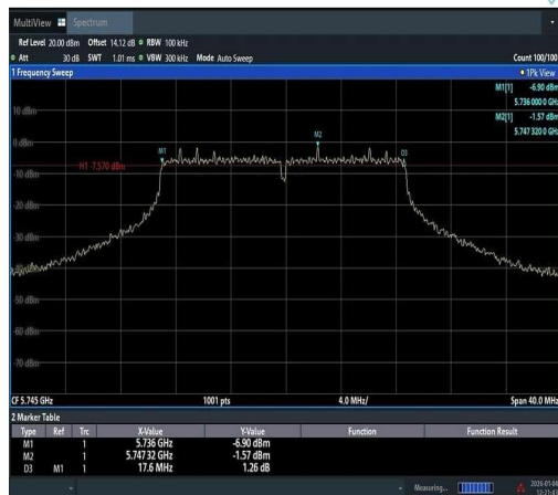
11AC20SISO-Ant1-5745-PASS
