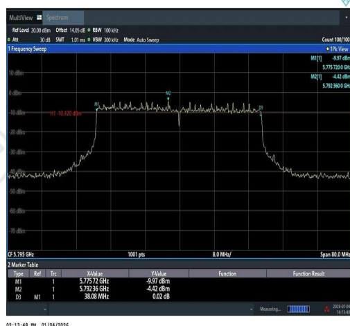
11AX40SISO-Ant1-5795-PASS
