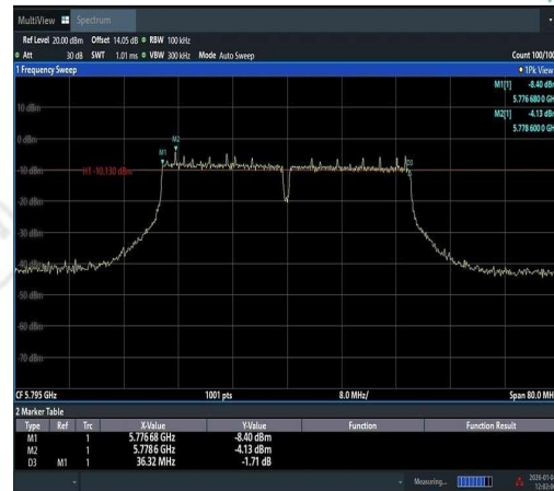
11N40SISO-Ant1-5795-PASS
