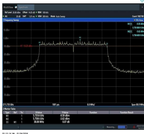
11AX40SISO-Ant1-5755-PASS
