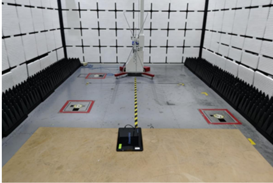
Radiated spurious emission Test Setup-1(Below 1GHz)
