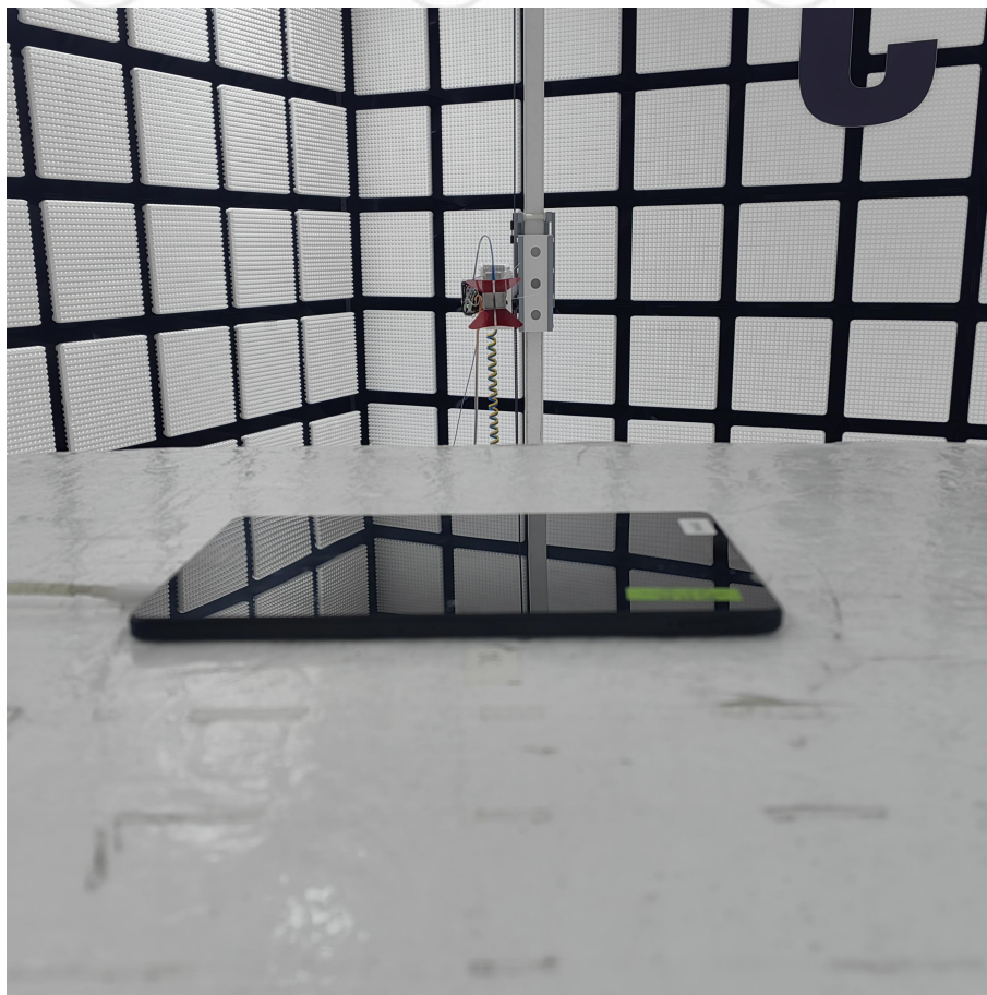
Radiated spurious emission Test Setup-4(Above 1GHz)
