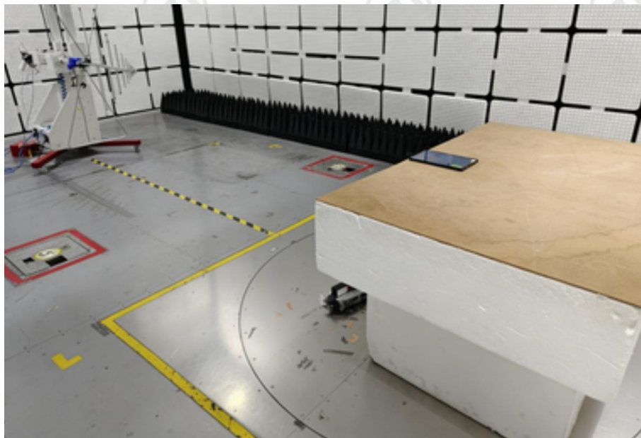
Radiated spurious emission Test Setup-2(Below 1GHz)
