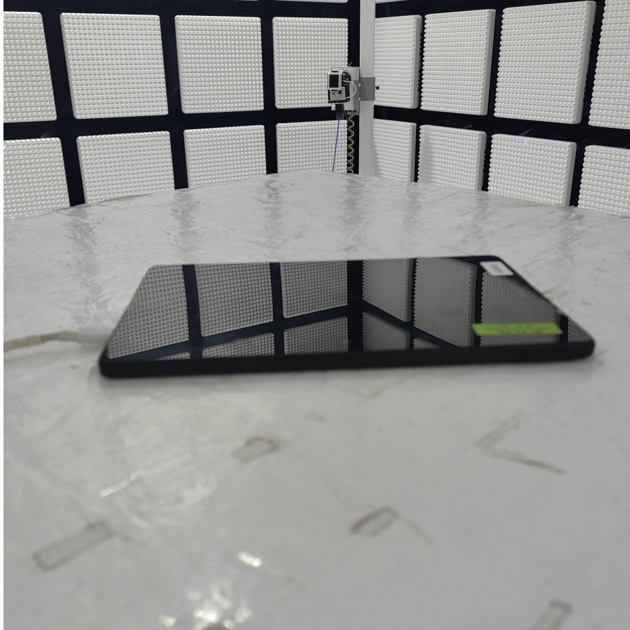
Radiated spurious emission Test Setup-5(Above 18GHz)
