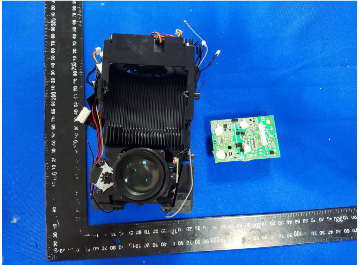
Internal photograph of EUT
