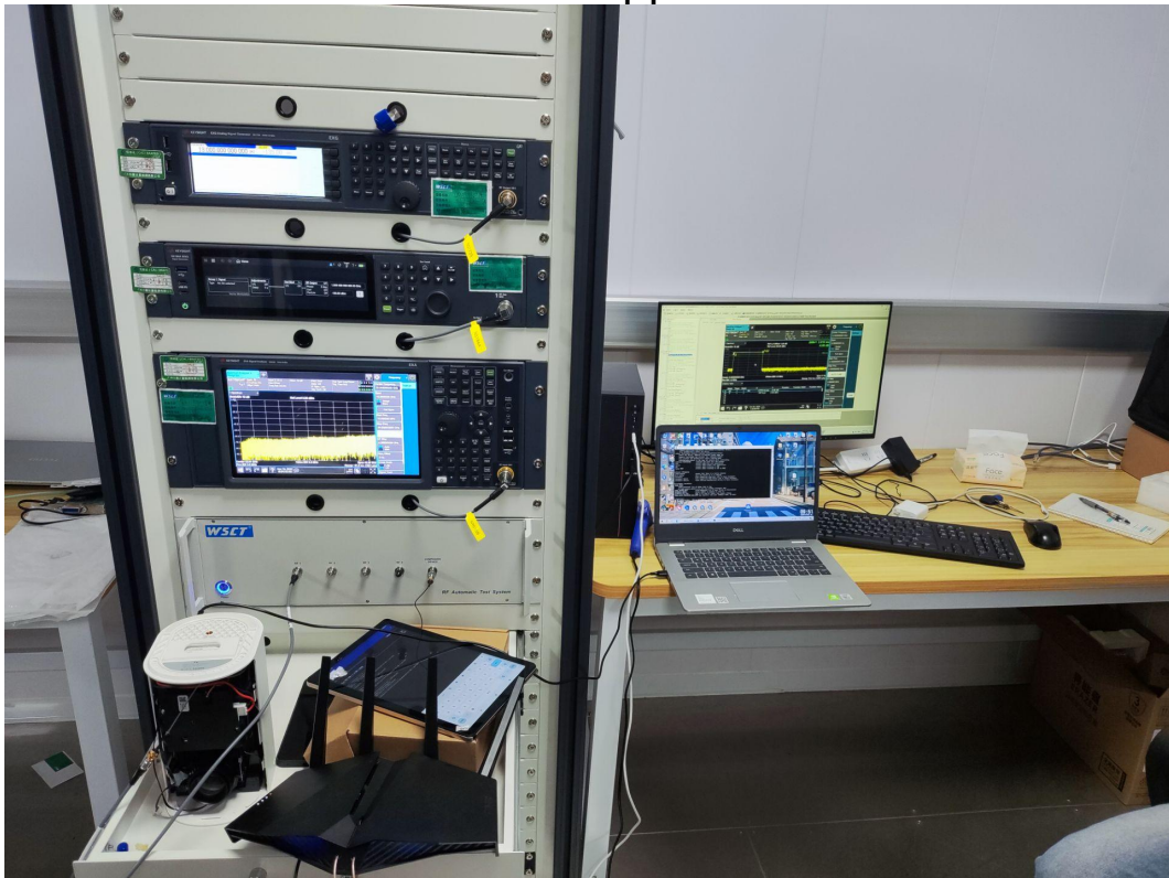
DFS Test setup photos
