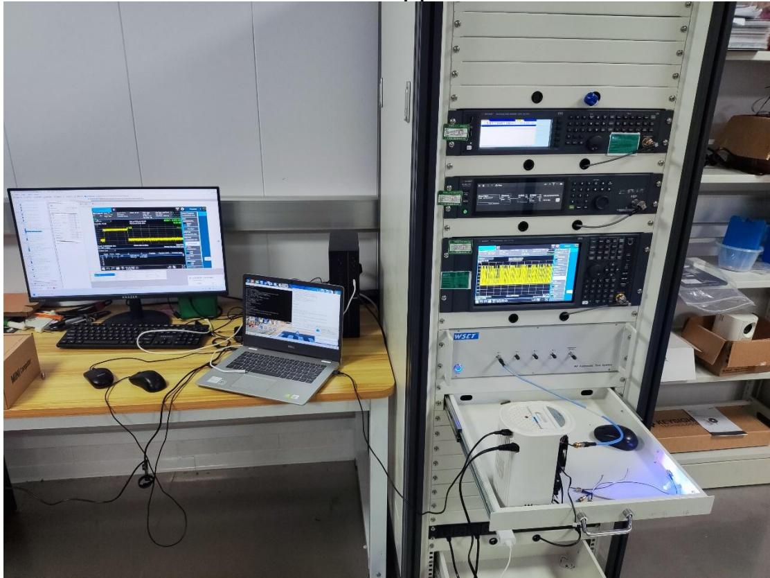
DFS Test setup photos
