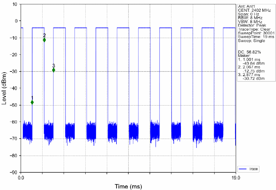
2M_LCH_2402MHz_Ant1_NTNV
