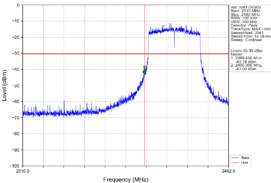
802.11ax(HEW40)_LCH_2422MHz_SU_/_Ant1 (SISO)_NTNV
