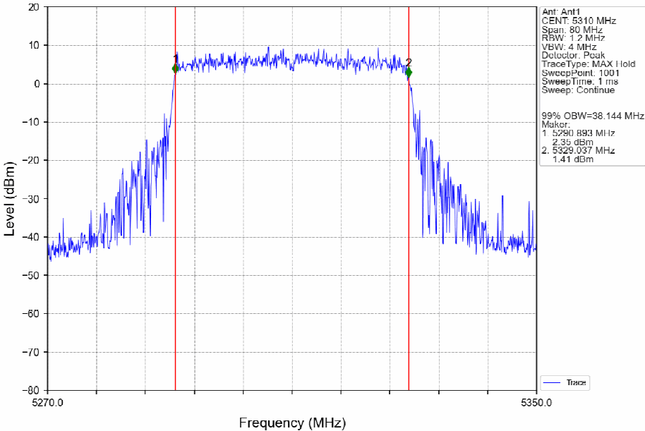
802.11ax(HEW40)_HCH_5310MHz_SU_/_Ant1_NTNV
