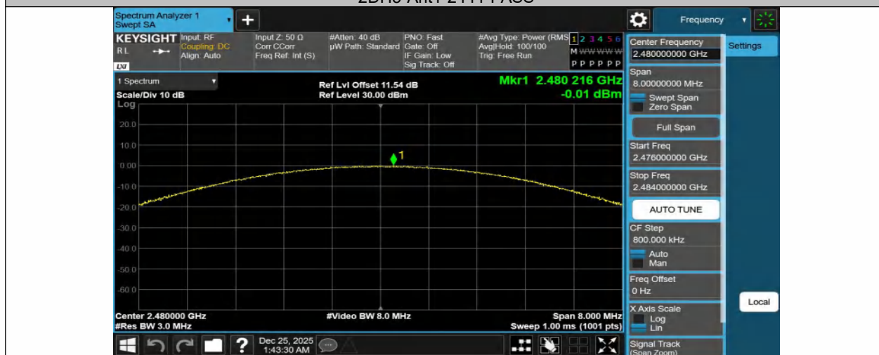
2DH5-Ant1-2480-PASS
