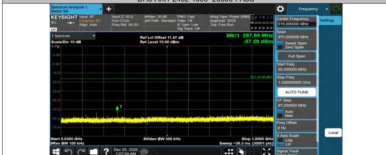
DH5-Ant1-2441-30~1000-PASS
