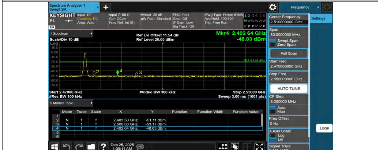
DH5-Ant1-2480-PASS
