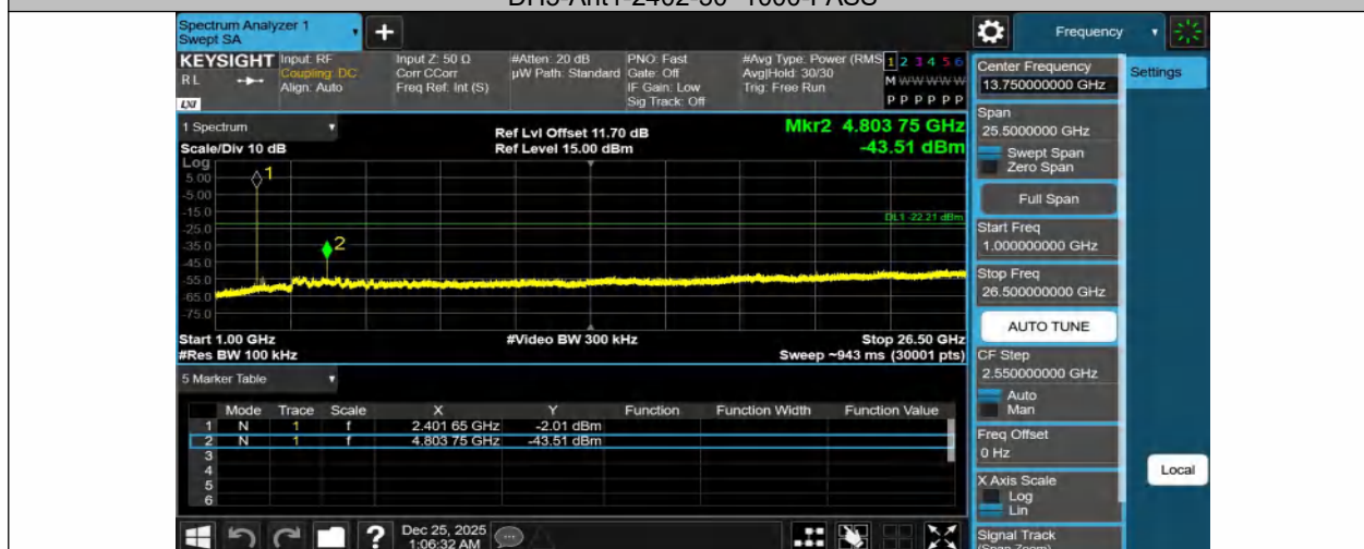
DH5-Ant1-2402-1000~26500-PASS
