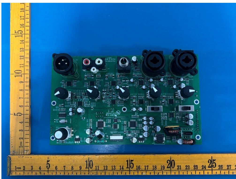
Internal view of unit (Model:POLAR 15 MK2)
