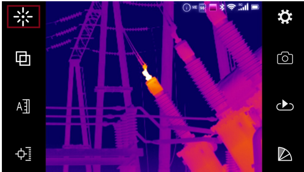
Laser ranging
