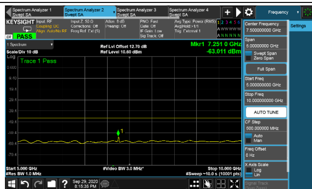
64QAM Middle channel
