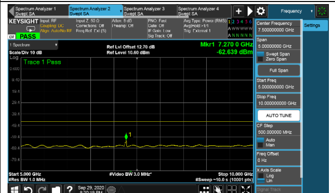
16QAM Middle channel
