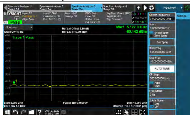
QPSK Middle channel
