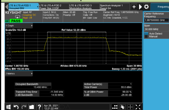
15MHz Channel Bandwidth - 256QAM
