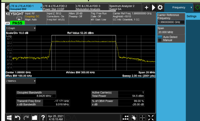
10MHz Channel Bandwidth - 256QAM
