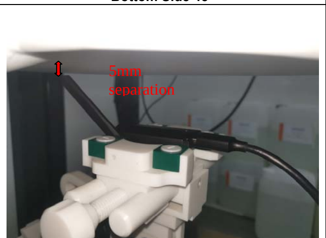
Bottom Side 120°
