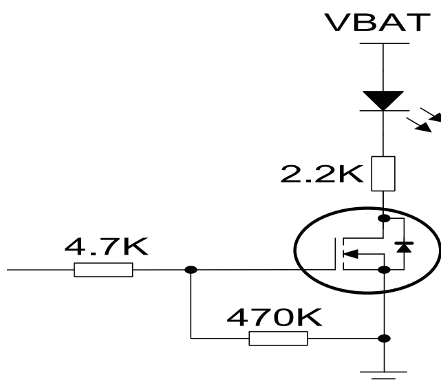
Figure 26: Reference Circuit of Network Status Indication
