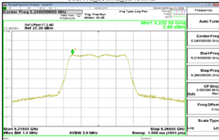
802.11a_20MHz_5240MHz
