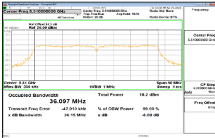
IC_802.11n_40MHz_Chain0_5510MHz
