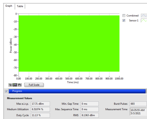
Figure 8.1-2: Maximum conducted power, 802.11n (SISO), mid channel
