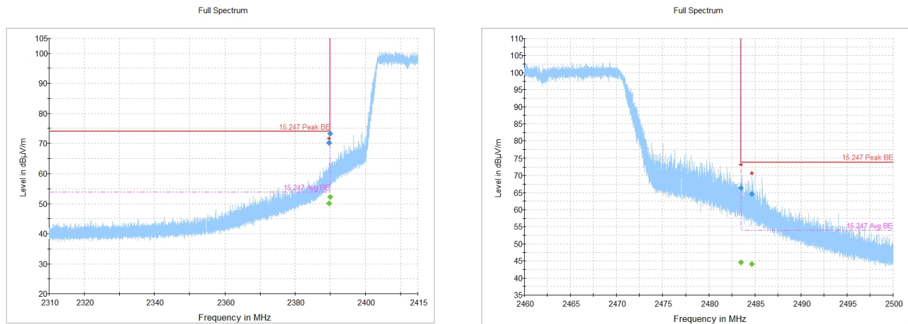
Figure 8.2-4: Radiated emissions, restricted band edge, 802.11ac, SISO antenna configuration
