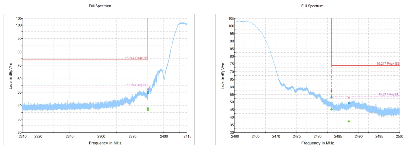
Figure 8.2-1: Radiated emissions, restricted band edge, 802.11b, SISO antenna configuration
