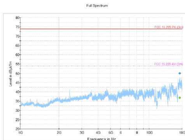
Figure 8.2-54: Radiated spurious emissions, 802.11ac MIMO 80MBW U-NII-2C Low channel
