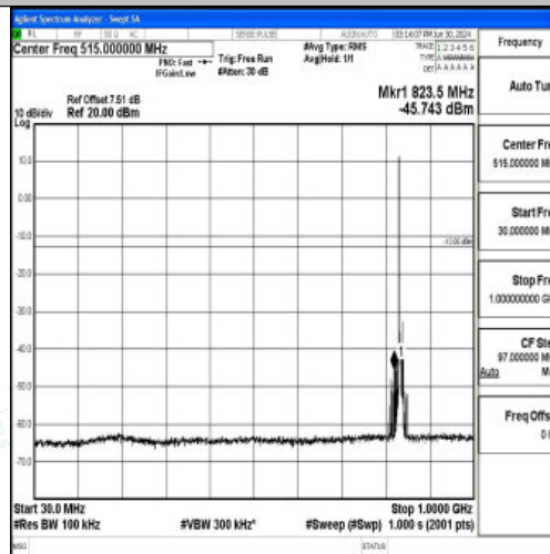
Band5_5MHz_QPSK_20525_1RB#0_30~1000_30~1000
