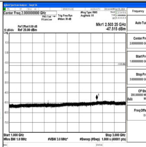
Band5_5MHz_16QAM_20525_1RB#0_1000~3000_1000~3000
