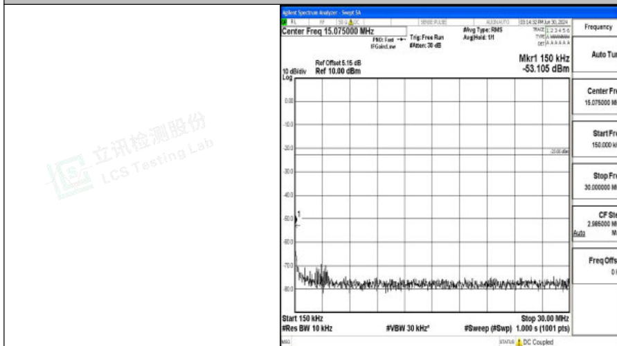
Band5_5MHz_16QAM_20525_1RB#0_0.15~30_0.15~30
