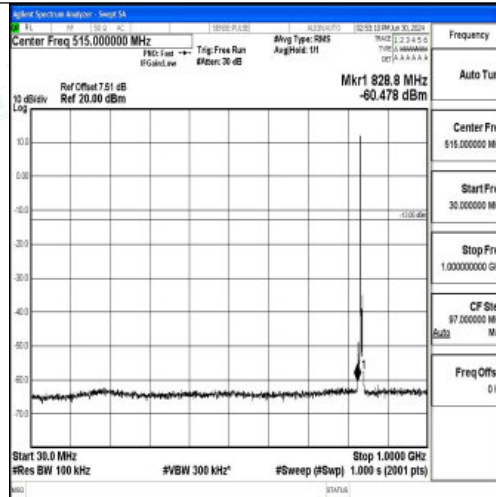
Band5_3MHz_16QAM_20525_1RB#0_30~1000_30~1000
