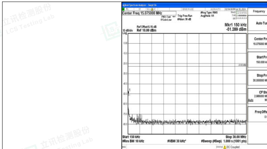
Band5_3MHz_16QAM_20635_1RB#0_0.15~30_0.15~30
