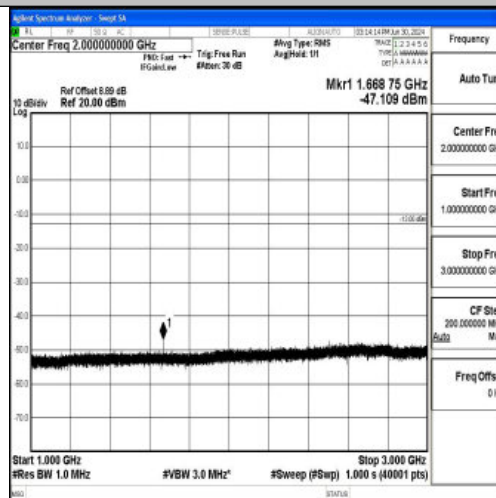
Band5_5MHz_QPSK_20525_1RB#0_1000~3000_1000~3000
