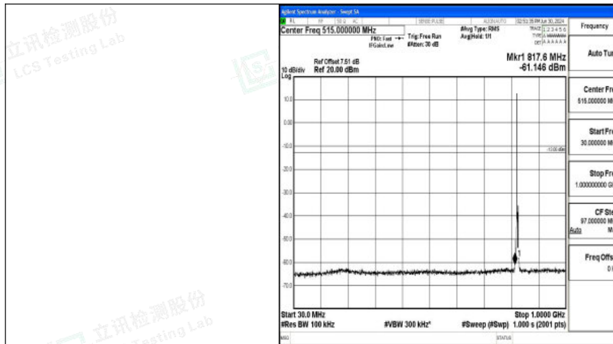
Band5_3MHz_QPSK_20415_1RB#0_30~1000_30~1000
