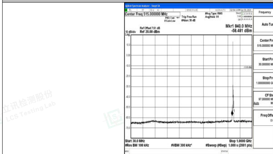
Band5_3MHz_16QAM_20635_1RB#0_30~1000_30~1000
