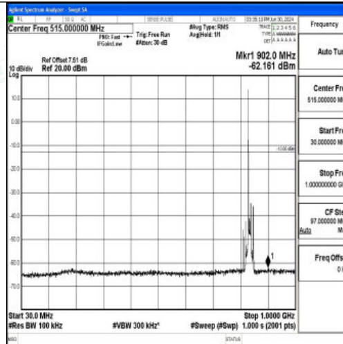
Band5_10MHz_16QAM_20525_1RB#0_30~1000_30~1000
