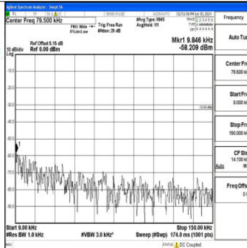
Band5_3MHz_16QAM_20415_1RB#0_0.009~0.15_0.009~0.15
