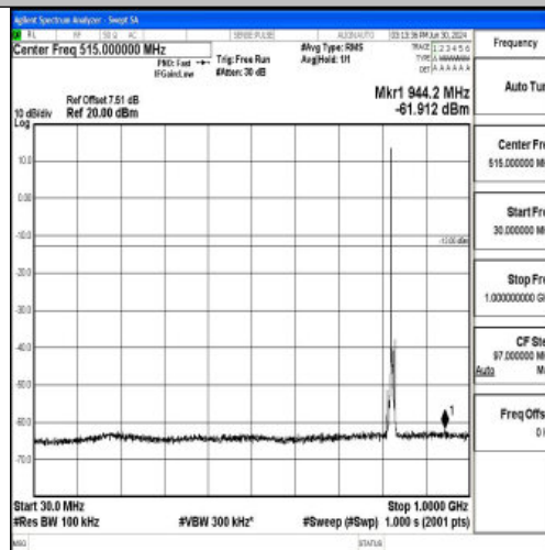
Band5_5MHz_16QAM_20425_1RB#0_30~1000_30~1000
