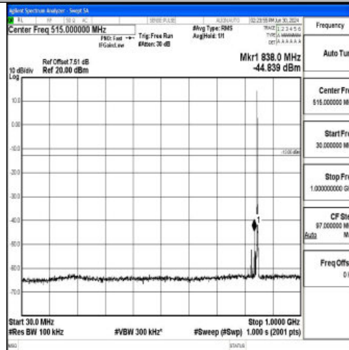
Band5_1.4MHz_QPSK_20643_1RB#0_30~1000_30~1000
