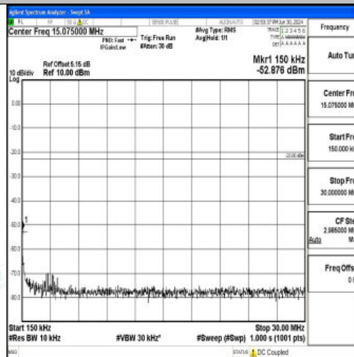
Band5_3MHz_QPSK_20635_1RB#0_0.15~30_0.15~30
