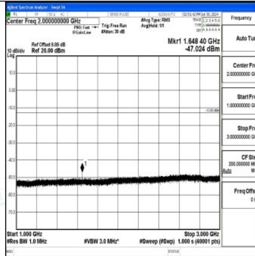
Band5_3MHz_QPSK_20415_1RB#0_1000~3000_1000~3000
