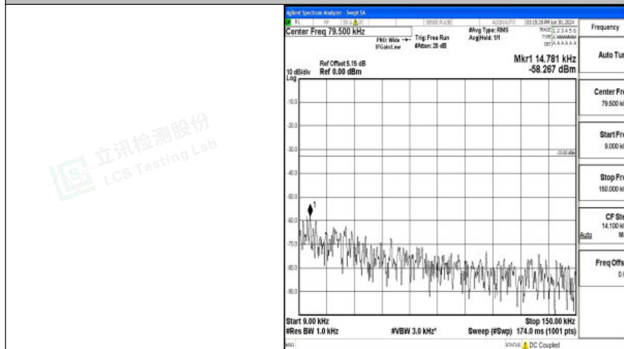
Band5_5MHz_16QAM_20625_1RB#0_0.009~0.15_0.009~0.15
