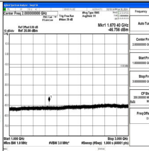
Band5_3MHz_16QAM_20525_1RB#0_1000~3000_1000~3000
