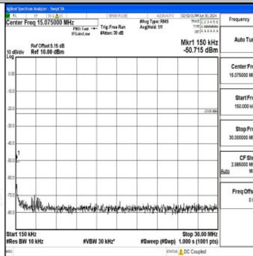
Band5_3MHz_16QAM_20415_1RB#0_0.15~30_0.15~30
