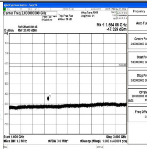
Band5_10MHz_16QAM_20525_1RB#0_1000~3000_1000~3000
