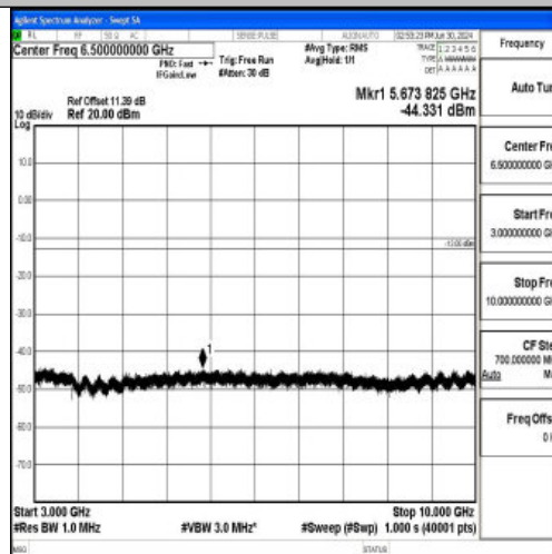
Band5_3MHz_16QAM_20525_1RB#0_3000~10000_3000~10000
