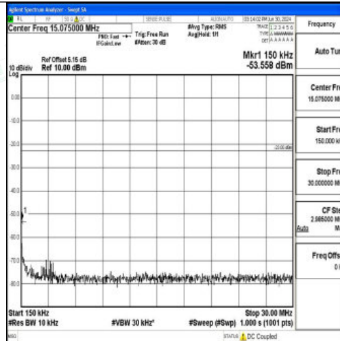
Band5_5MHz_QPSK_20525_1RB#0_0.15~30_0.15~30
