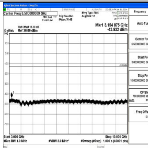
Band5_10MHz_16QAM_20525_1RB#0_3000~10000_3000~10000
