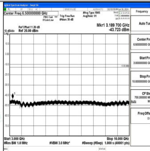
Band5_3MHz_QPSK_20635_1RB#0_3000~10000_3000~10000
