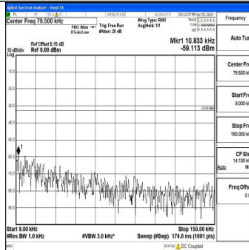
Band5_5MHz_QPSK_20525_1RB#0_0.009~0.15_0.009~0.15
