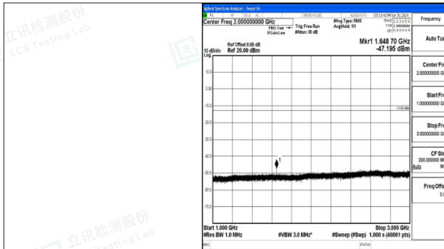
Band5_5MHz_16QAM_20425_1RB#0_1000~3000_1000~3000
