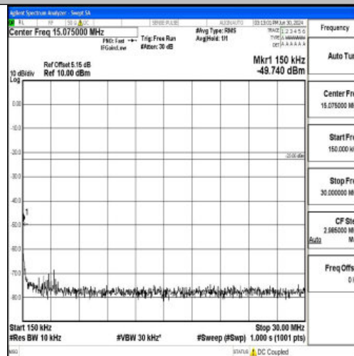
Band5_5MHz_QPSK_20425_1RB#0_0.15~30_0.15~30
