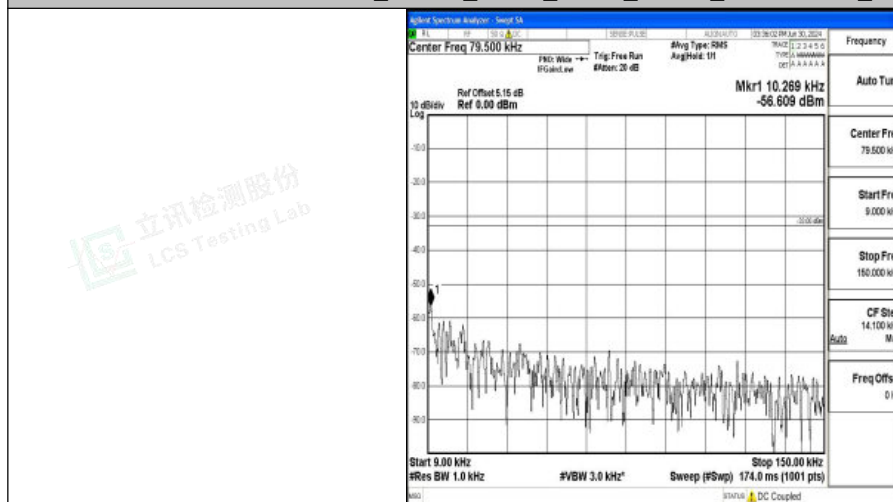
Band5_10MHz_16QAM_20600_1RB#0_0.009~0.15_0.009~0.15
