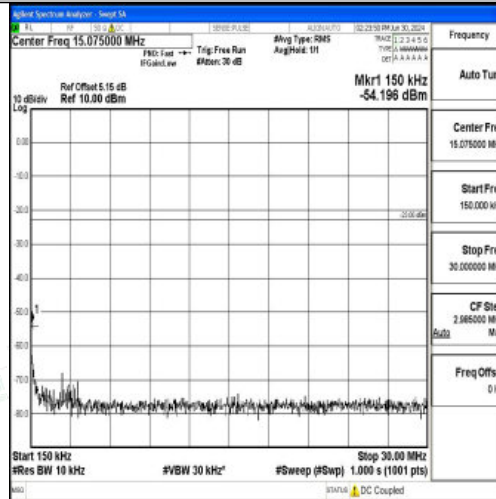
Band5_1.4MHz_QPSK_20643_1RB#0_0.15~30_0.15~30
