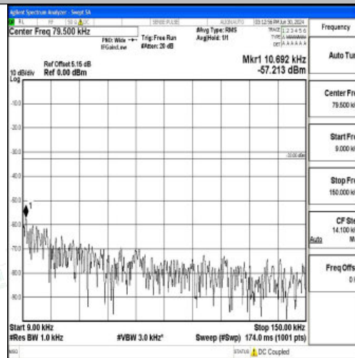
Band5_5MHz_QPSK_20425_1RB#0_0.009~0.15_0.009~0.15
