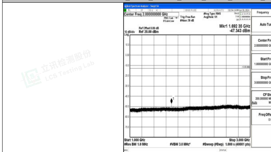
Band5_3MHz_16QAM_20635_1RB#0_1000~3000_1000~3000
