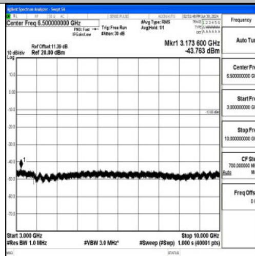
Band5_3MHz_QPSK_20415_1RB#0_3000~10000_3000~10000
