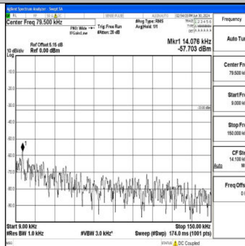
Band5_3MHz_16QAM_20635_1RB#0_0.009~0.15_0.009~0.15
