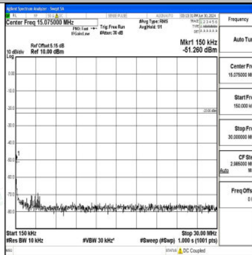
Band5_5MHz_16QAM_20425_1RB#0_0.15~30_0.15~30
