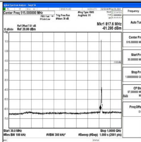
Band5_3MHz_16QAM_20415_1RB#0_30~1000_30~1000
