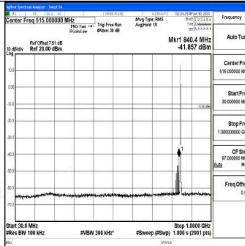
Band5_1.4MHz_16QAM_20643_1RB#0_30~1000_30~1000
