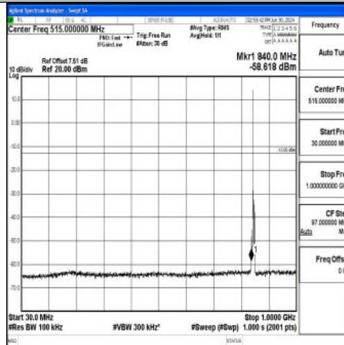
Band5_3MHz_QPSK_20635_1RB#0_30~1000_30~1000
