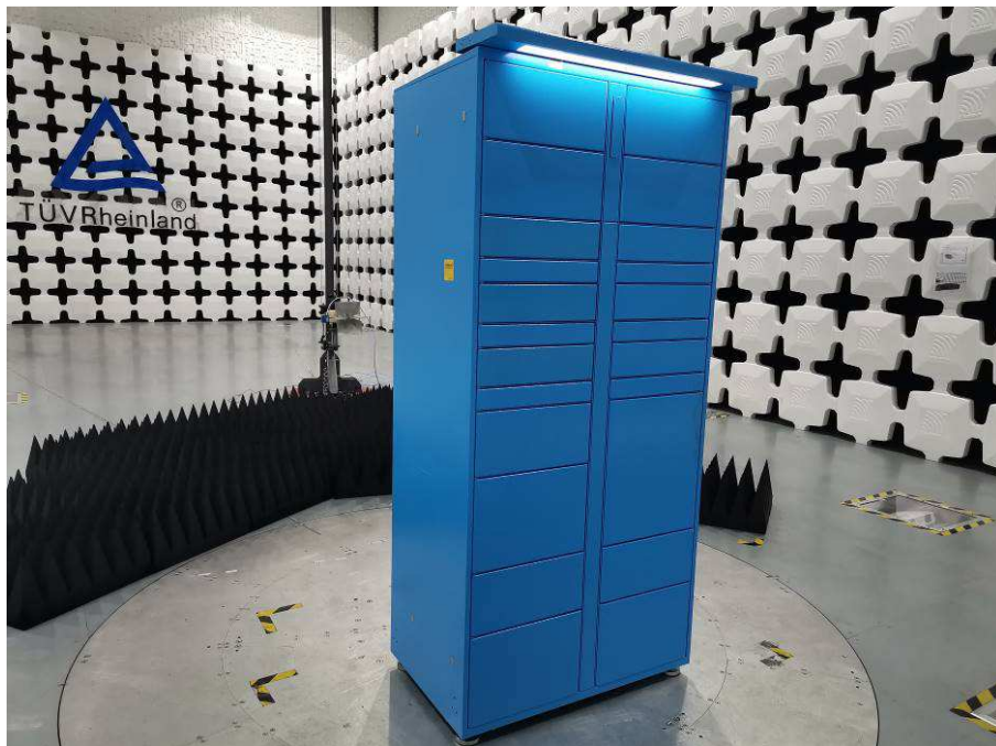
Photograph 2: Set-up photo for Radiated Emission, Above 1GHz
