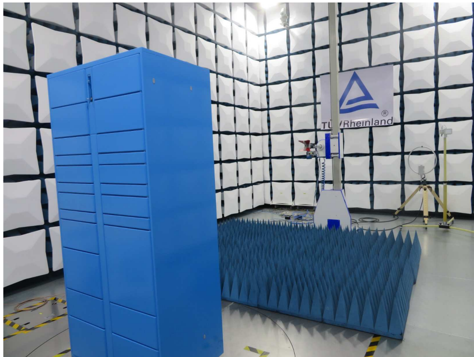
Photograph 1: Set-up for License Radio and Co-Located Radiated Spurious Emissions
