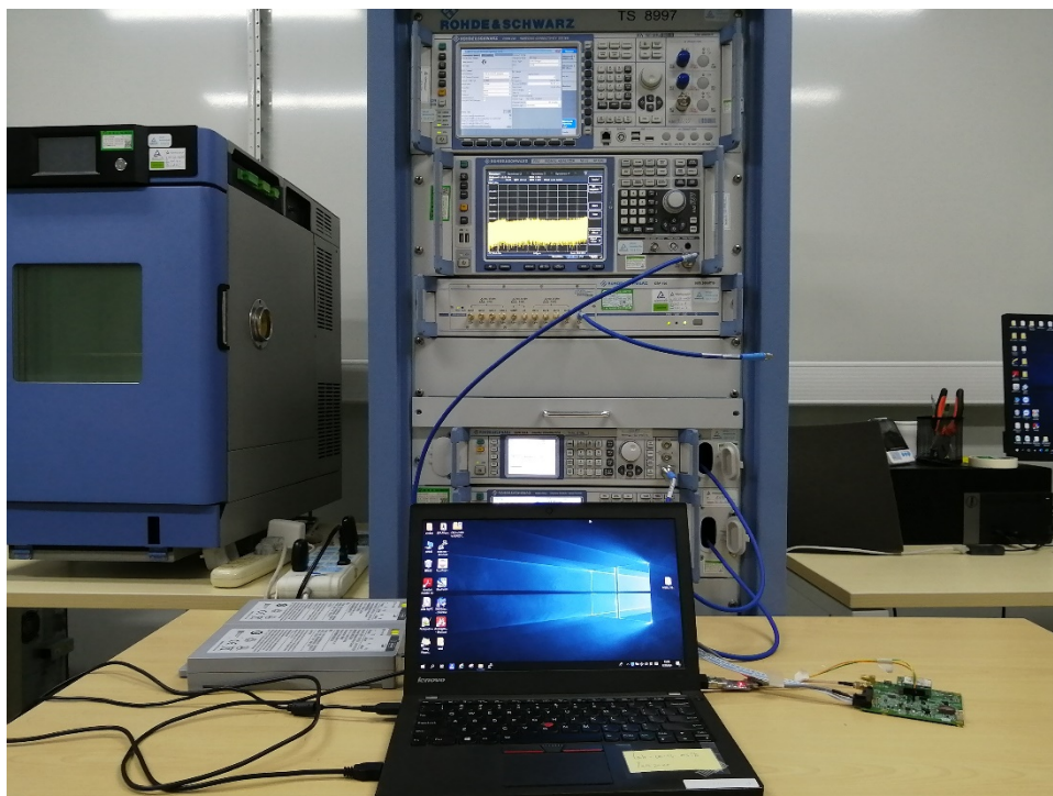
Photograph 2: Set-up for Conducted Measurements
