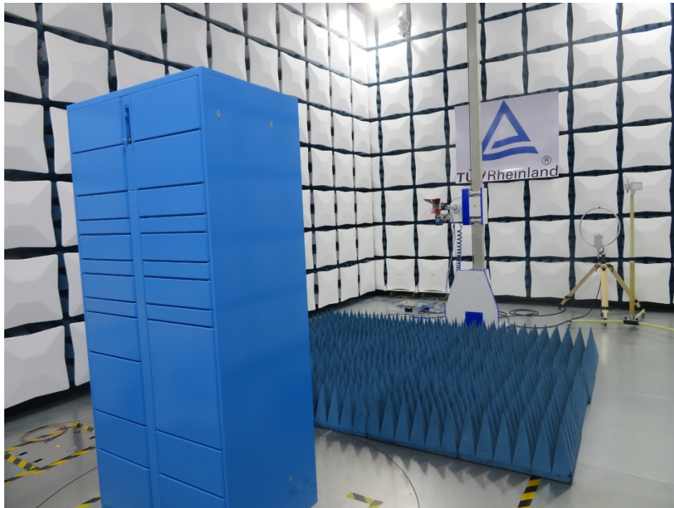
Photograph 1: Set-up for Radiated Spurious Emission
