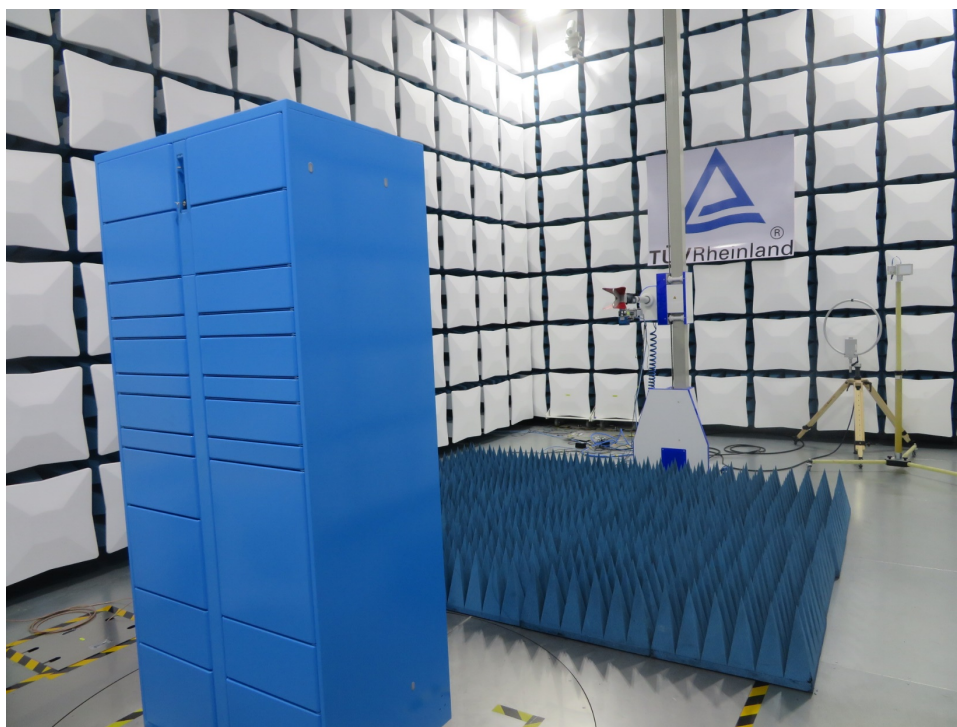
Photograph 1: Set-up for License Radio and Co-Located Radiated Spurious Emissions
