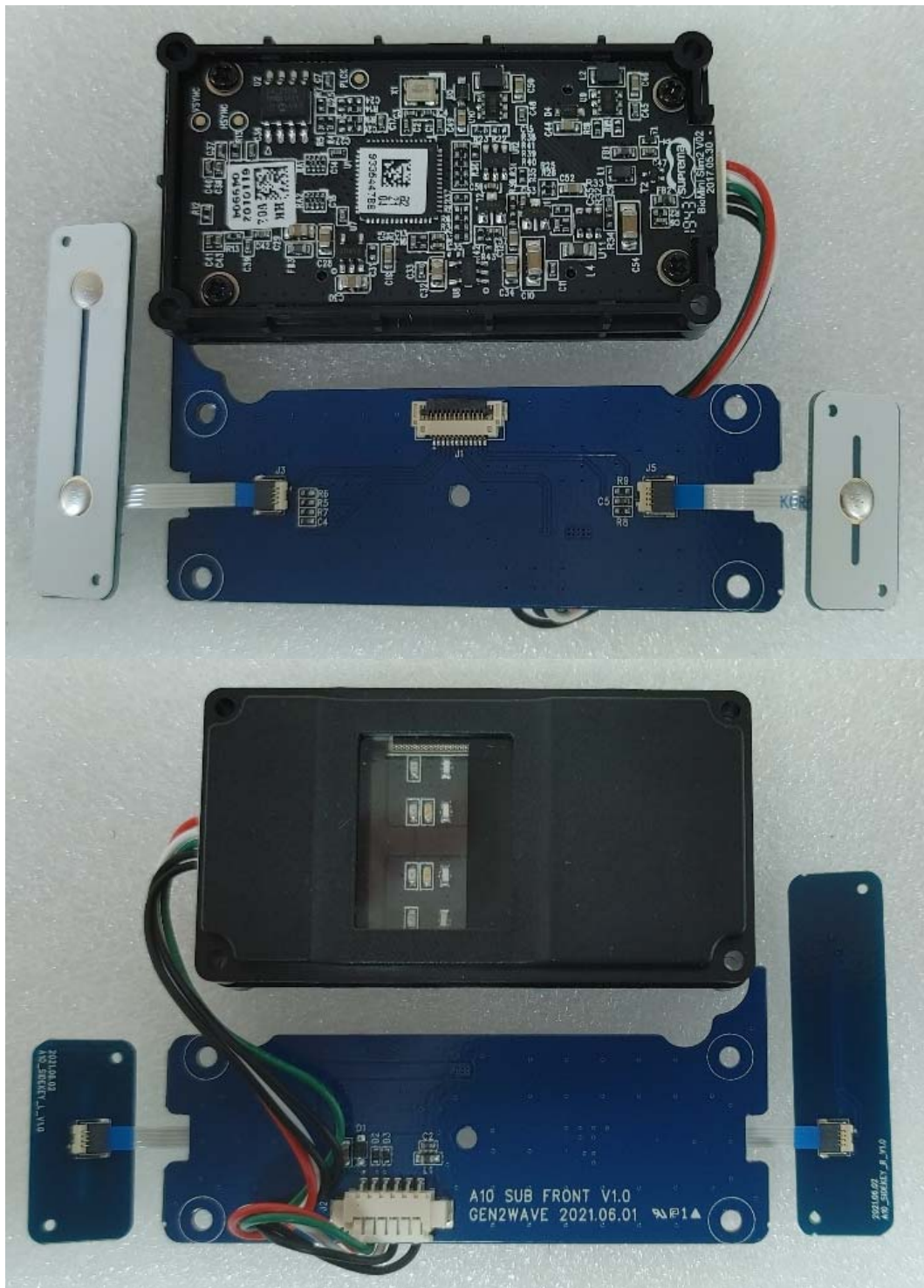
< SUB FRONT board >
