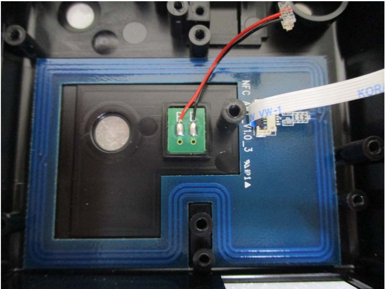
< RFID 1 (ACM1281U) Antenna >
