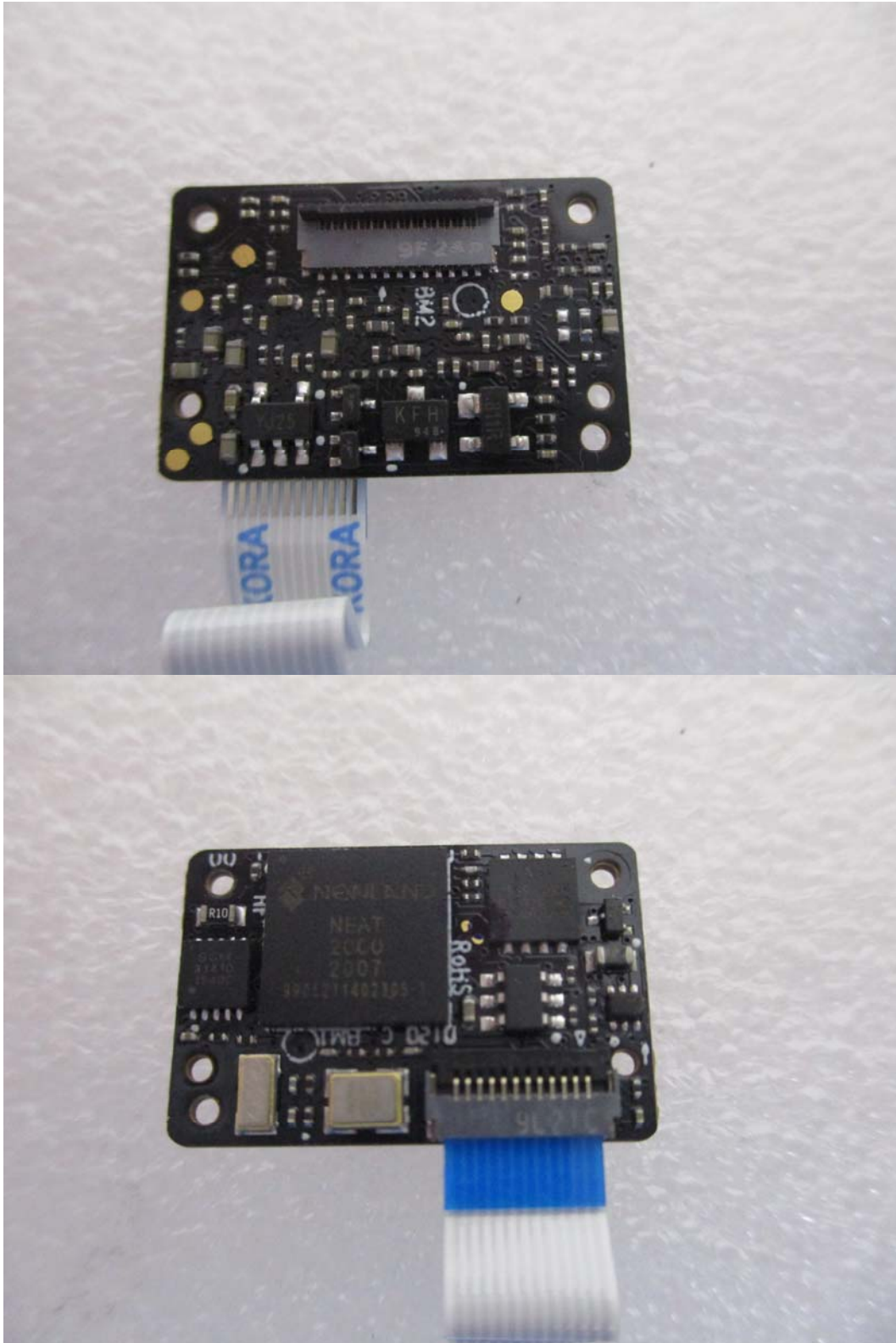
< Sub board >
