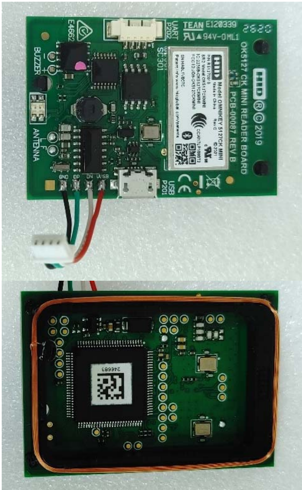
< HID board –RFID 2 >
