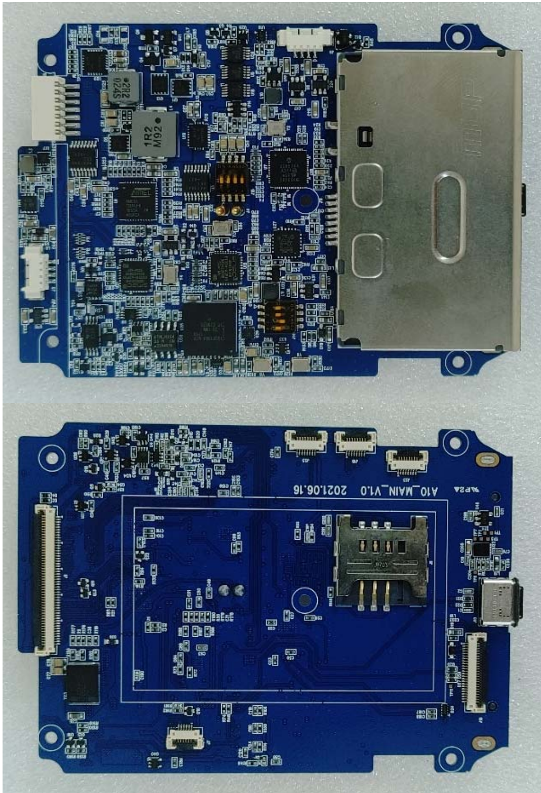
< Main board >
