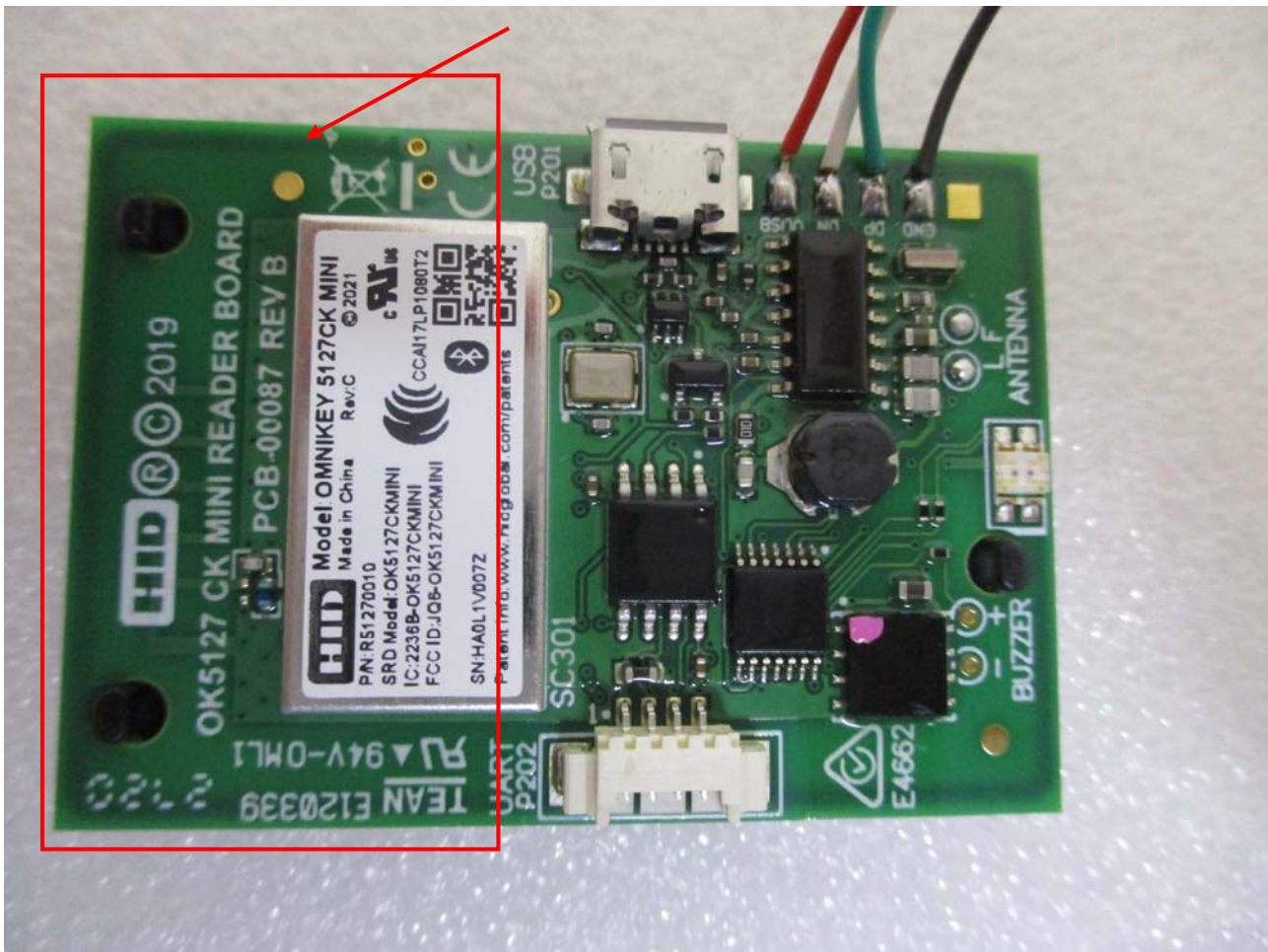
< RFID 2(HID) -13.56 MHz Antenna >
