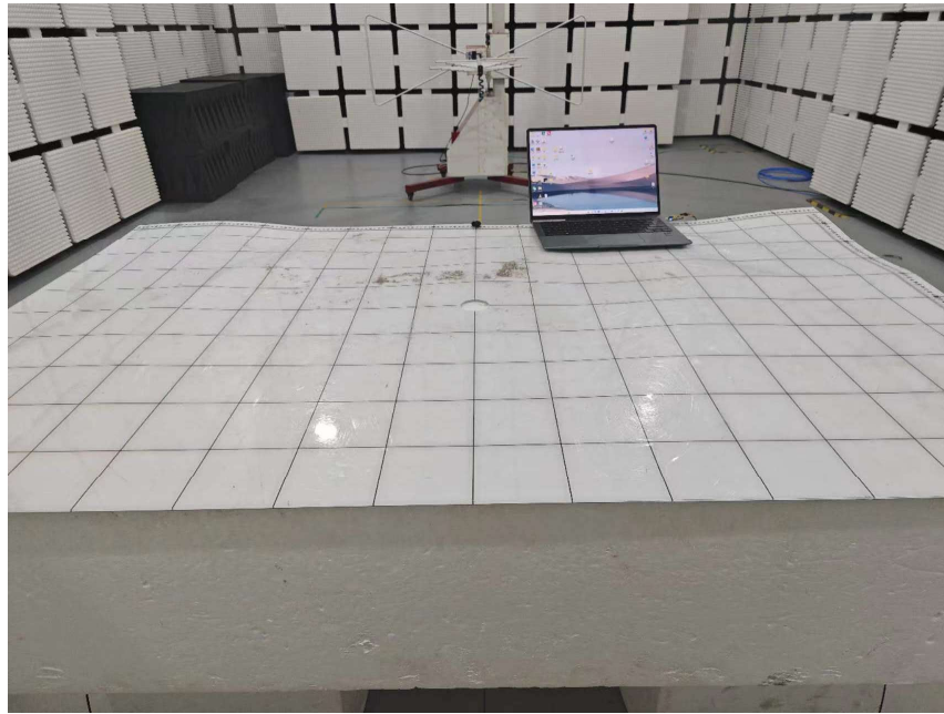
Set-up for Radiated Spurious Emission, Above 1GHz(Right earphone)
