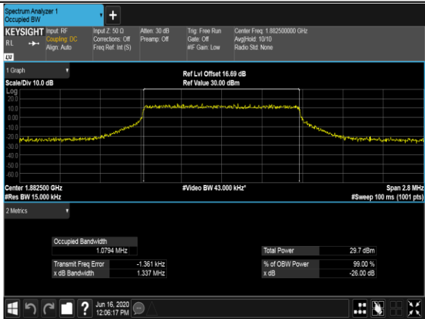
MCH_QPSK_6RB#0
