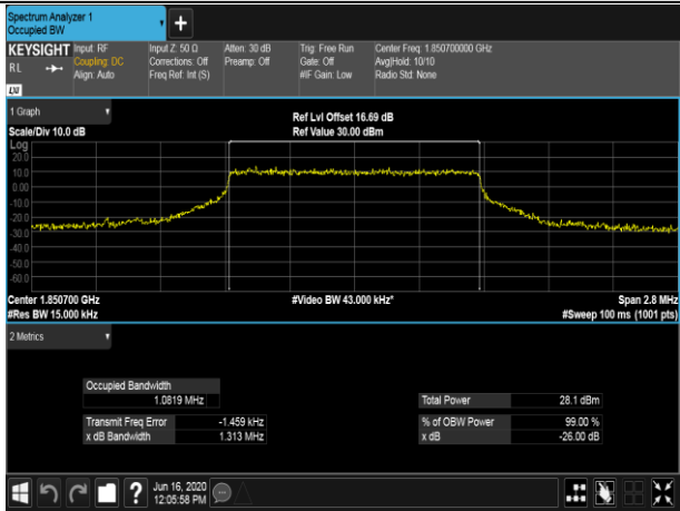
LCH_QPSK_6RB#0
