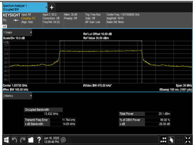
LCH_16QAM_75RB#0
