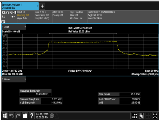
LCH_QPSK_75RB#0
