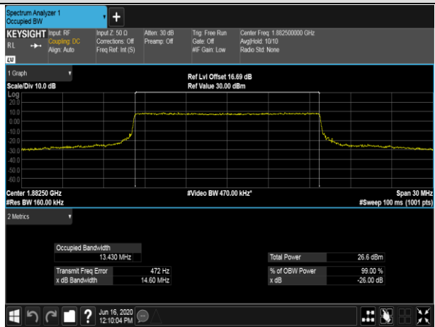
MCH_16QAM_75RB#0
