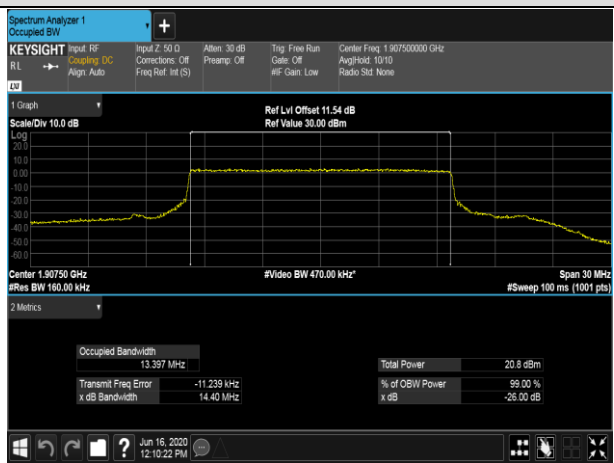
HCH_16QAM_75RB#0
