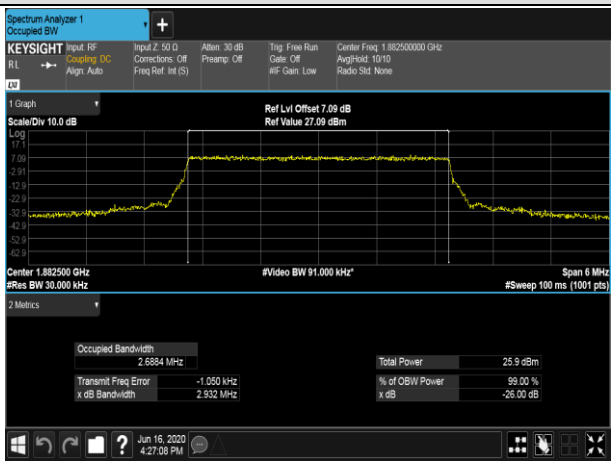
MCH_QPSK_15RB#0
