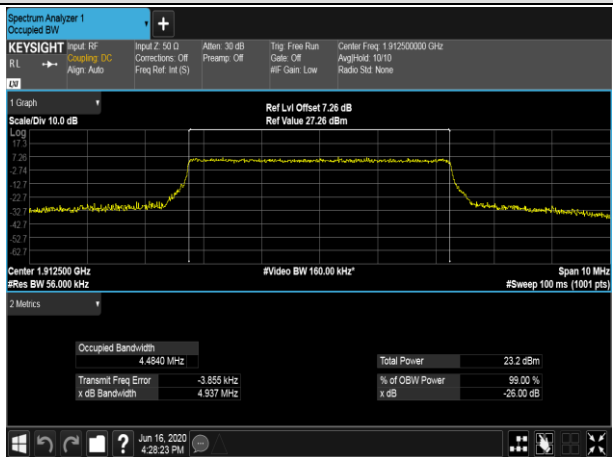
HCH_16QAM_25RB#0
