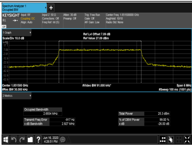
LCH_QPSK_15RB#0
