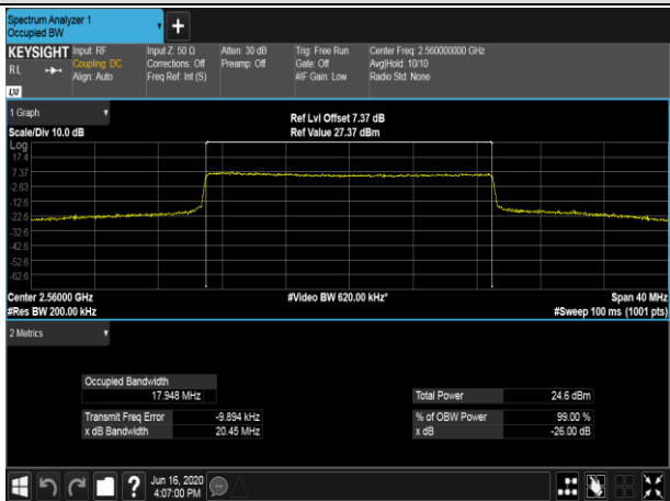
HCH_QPSK_100RB#0
