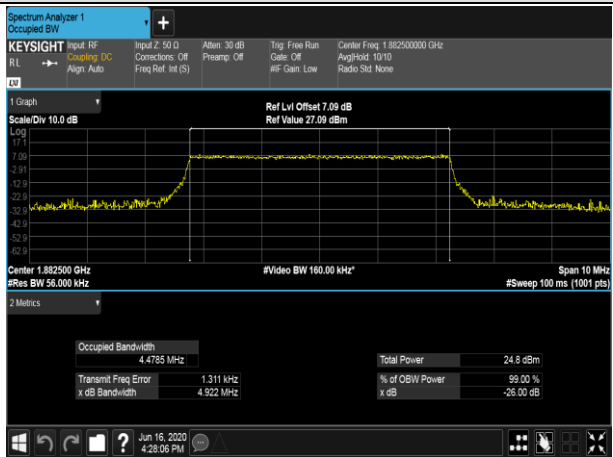
MCH_16QAM_25RB#0
