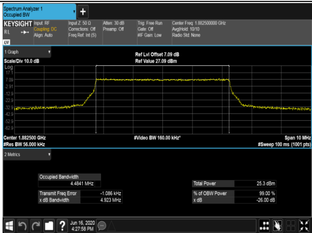
MCH_QPSK_25RB#0
