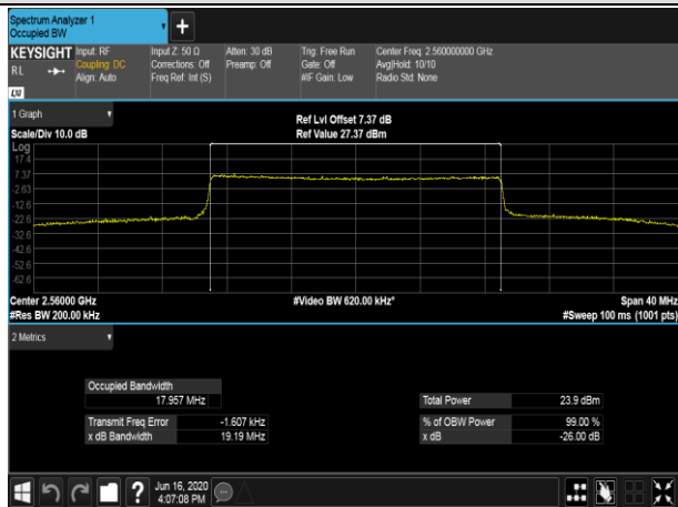
HCH_16QAM_100RB#0
