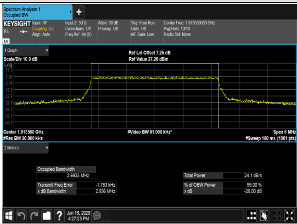
HCH_QPSK_15RB#0
