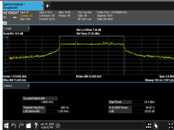
HCH_16QAM_6RB#0
