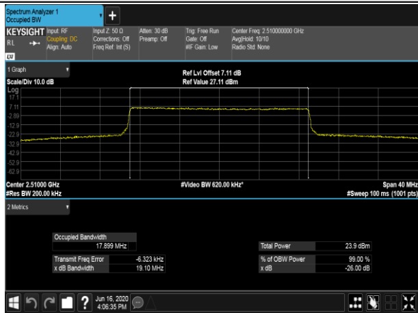
LCH_16QAM_100RB#0
