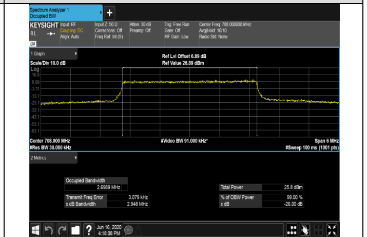
MCH_16QAM_15RB#0
