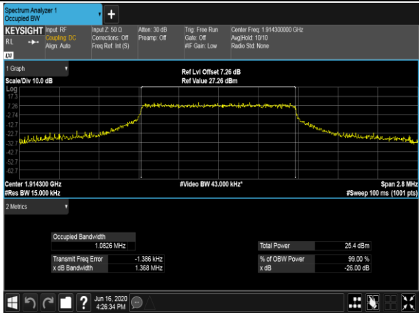
HCH_QPSK_6RB#0
