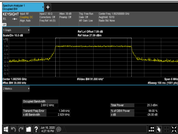
MCH_16QAM_15RB#0
