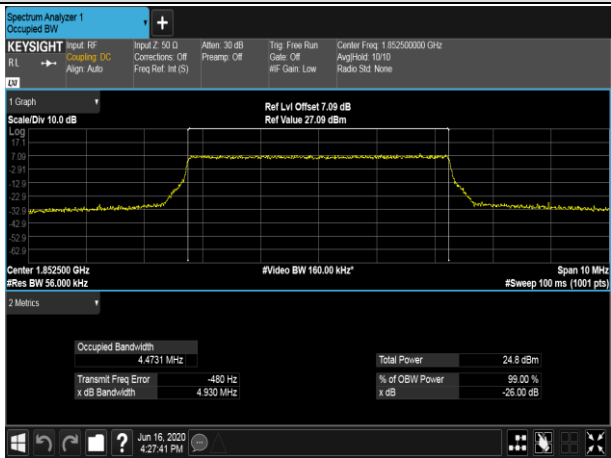
LCH_QPSK_25RB#0
