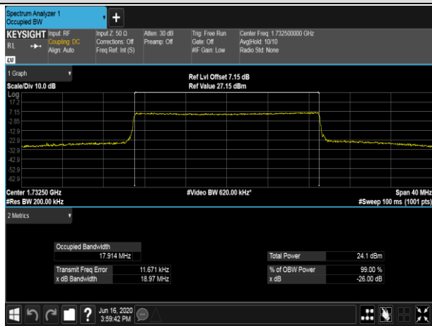
MCH_16QAM_100RB#0
