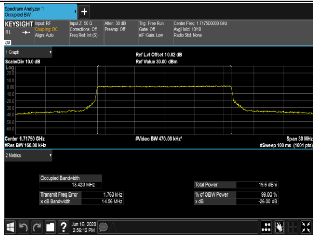
LCH_16QAM_75RB#0
