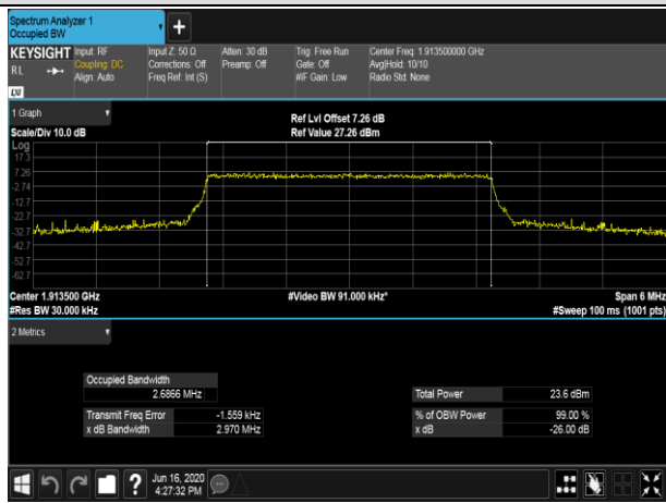
HCH_16QAM_15RB#0
