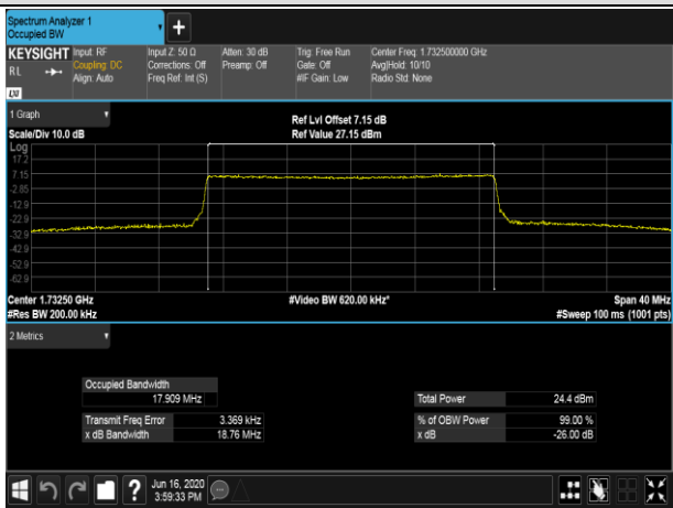
MCH_QPSK_100RB#0
