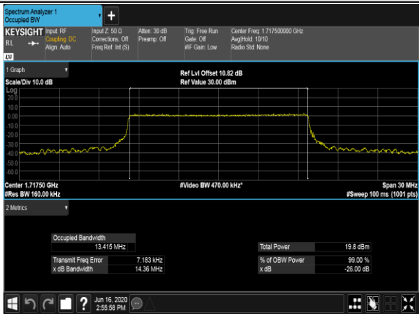
LCH_QPSK_75RB#0
