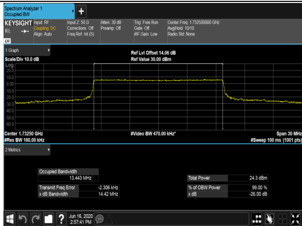
MCH_16QAM_75RB#0
