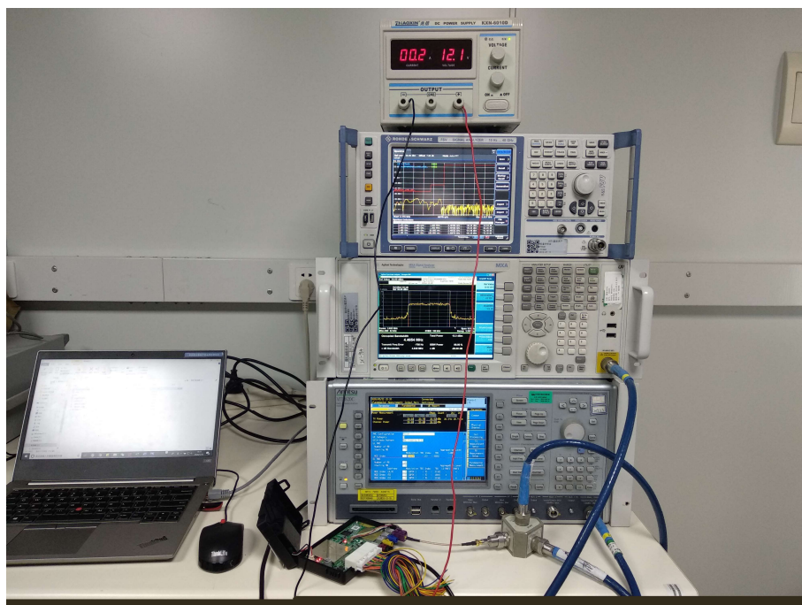
RF Conducted Test setup (CDMA/LTE)
