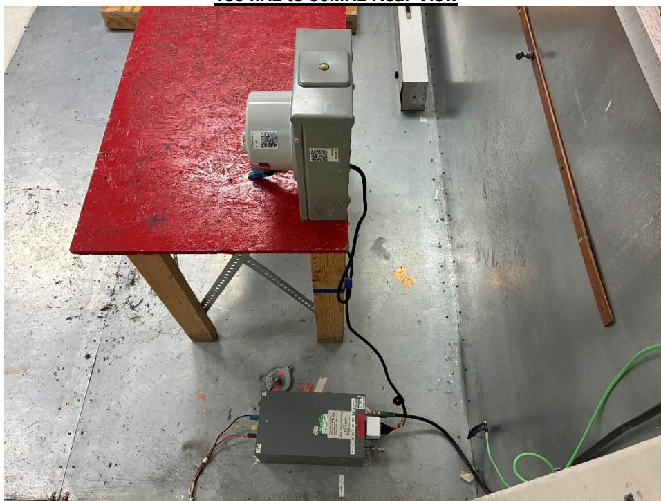
150 kHz to 30MHz Rear View
