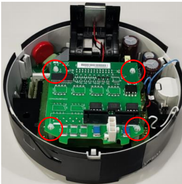
KYZ board_26 pin connector
