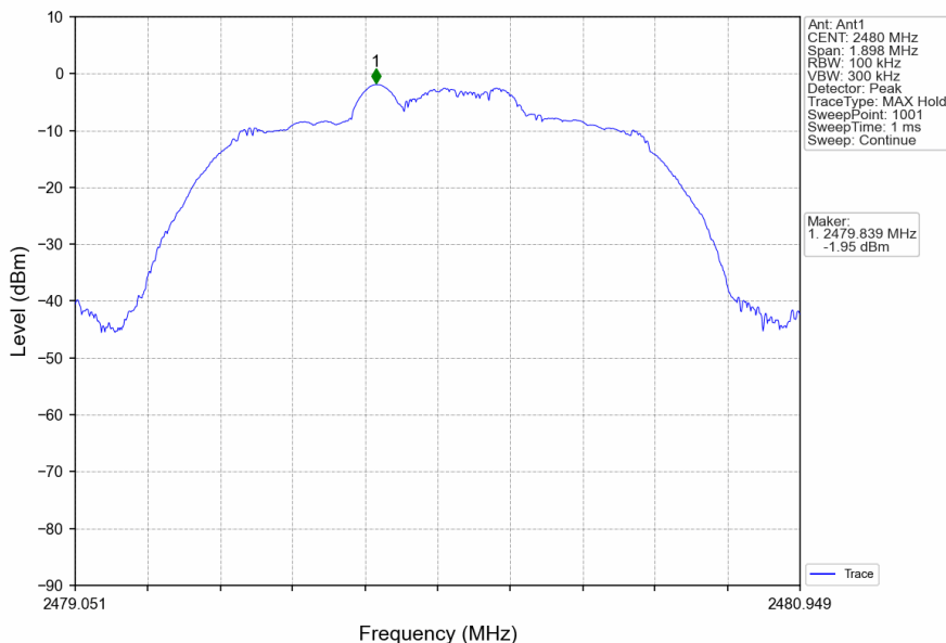
Pi/4DQPSK_2DH5_HCH_2480MHz_Ant1_NTNV
