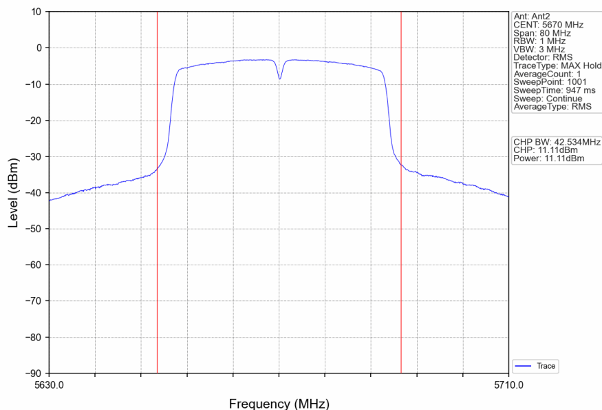
802.11n(HT40)_HCH_5670MHz_Ant2_NTNV
