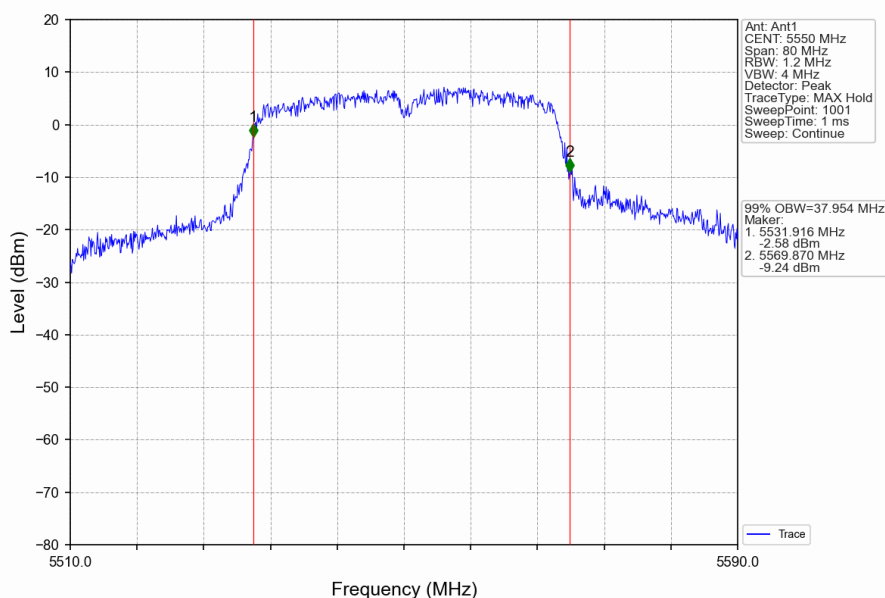
802.11n(HT40)_MCH_5550MHz_Ant1_NTNV
