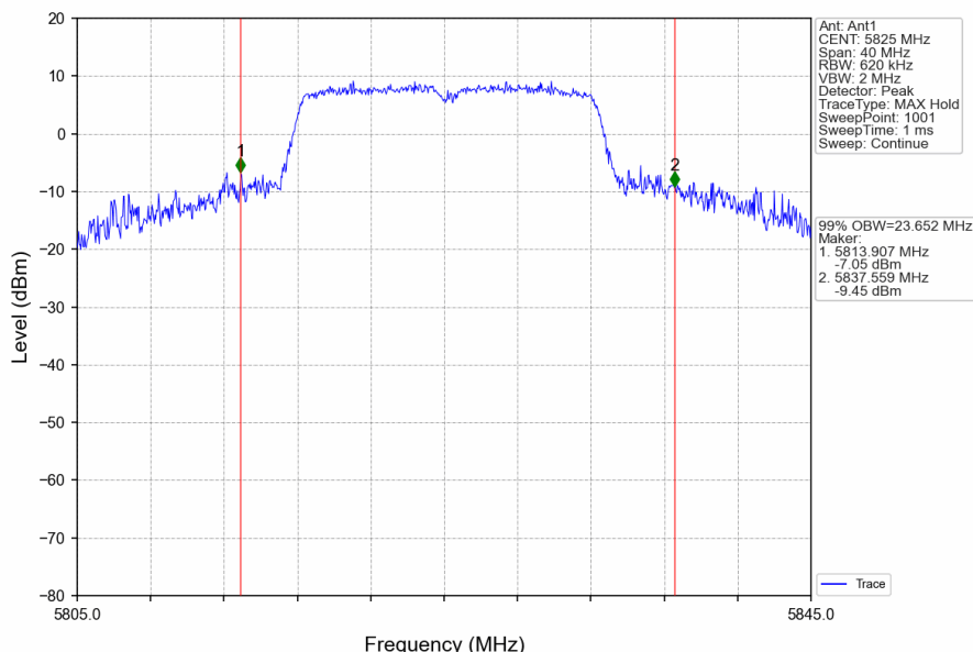
802.11a_HCH_5825MHz_Ant1_NTNV
